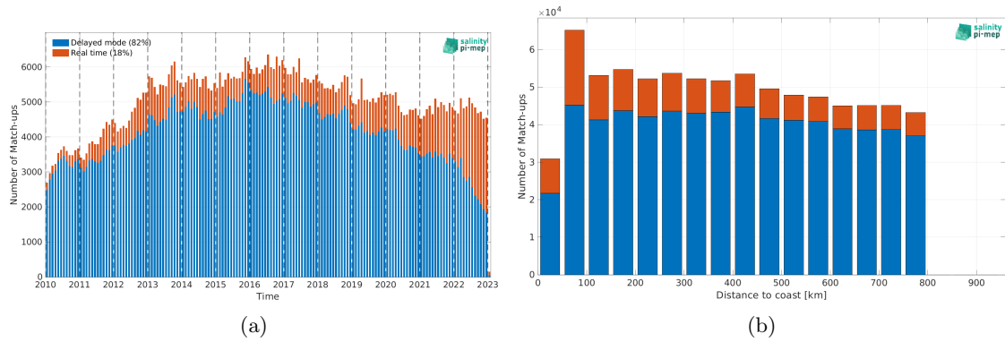
Figure 1: Number of match-ups between Argo and SMOS SSS L3 v8 - 9 Days (CATDS-CEC-LOCEAN) SSS as a function of time (a) and as function of the distance to coast (b) over the SMOS coastal zone (<800km) 60N-60S Pi-MEP region and for the full satellite product period.
