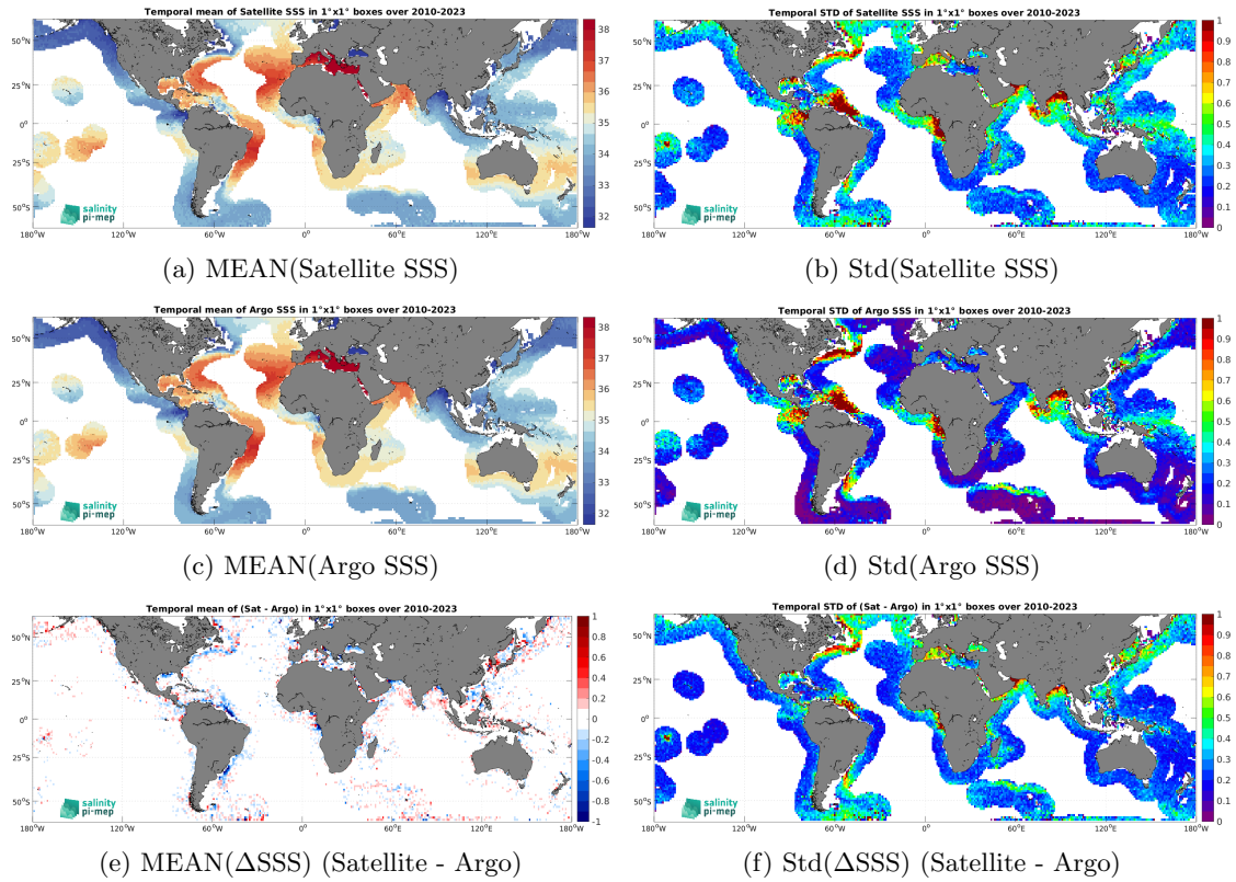
Figure 6: Temporal mean (left) and Std (right) of SSS from SMOS SSS L3 v8 - 9 Days (CATDS-CEC-LOCEAN) (top), Argo (middle), and of \Delta SSS (Satellite - Argo). Only match-up pairs are used to generate these maps.
