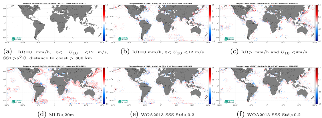
Figure 12: Temporal mean gridded over spatial boxes of size 1^\circ \times 1^\circ of \Delta SSS (SMOS SSS L3 v8 - 9 Days (CATDS-CEC-LOCEAN) - Argo) for 6 different subdatasets corresponding to:RR=0 mm/h, 3 < U_{10} < 12 m/s, SST >5^\circ C, distance to coast > 800 km (a), RR=0 mm/h, 3 < U_{10} < 12 m/s (b), RR >1 mm/h and U_{10} < 4 m/s (c),MLD <20 m (d),WOA2013 SSS Std <0.2 (e),WOA2013 SSS Std >0.2 (f).
