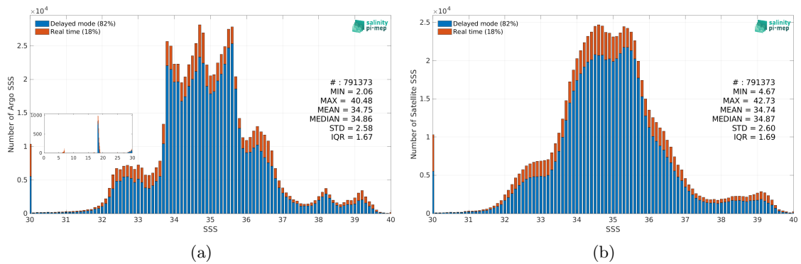
Figure 2: Histograms of SSS from Argo (a) and SMOS SSS L3 v8 - 9 Days (CATDS-CEC-LOCEAN) (b) considering all match-up pairs per bins of 0.1 over the SMOS coastal zone (<800km) 60N-60S Pi-MEP region and for the full satellite product period.
