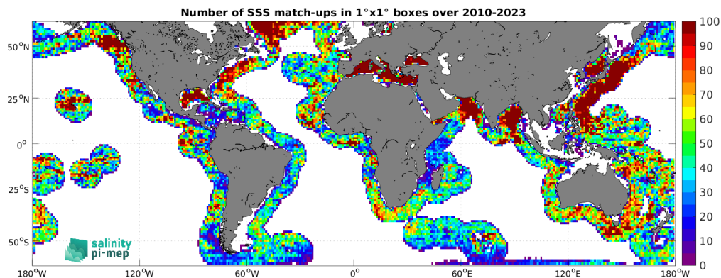
Figure 4: Number of SSS match-ups between Argo SSS and the SMOS SSS L3 v8 - 9 Days (CATDS-CEC-LOCEAN) SSS product for the SMOS coastal zone (<800km) 60N-60S Pi-MEP region over 1^\circ \times 1^\circ boxes and for the full satellite product period.
