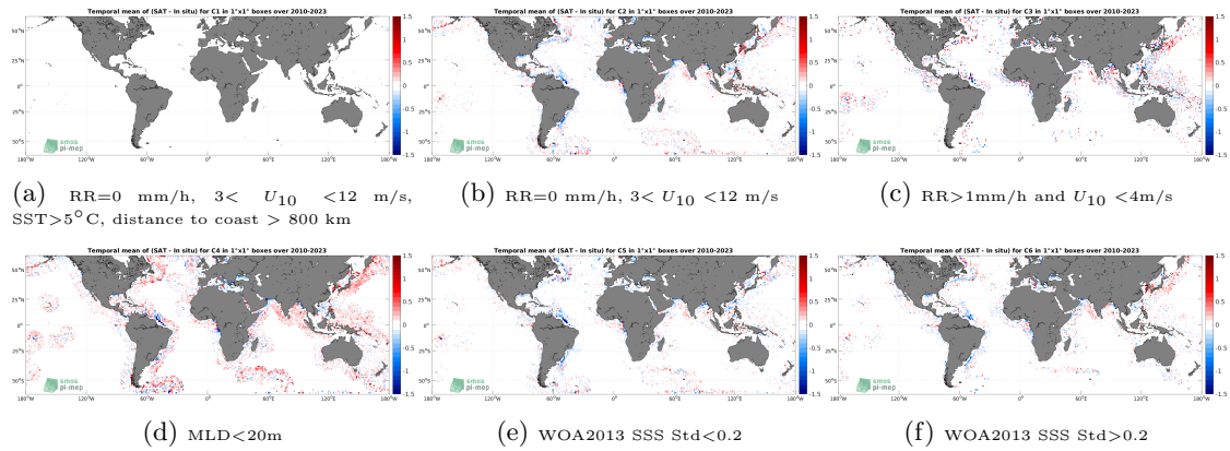
Figure 12: Temporal mean gridded over spatial boxes of size 1^\circ \times 1^\circ of \Delta SSS (SMOS SSS L3 v8 - 9 Days (CATDS-CECOS-LOCEAN) - Argo) for 6 different subdatasets corresponding to:RR=0 mm/h, 3 < U_{10} < 12 m/s, SST >5^\circ C, distance to coast > 800 km (a), RR=0 mm/h, 3 < U_{10} < 12 m/s (b), RR >1 mm/h and U_{10} < 4 m/s (c),MLD <20 m (d),WOA2013 SSS Std <0.2 (e),WOA2013 SSS Std >0.2 (f).
