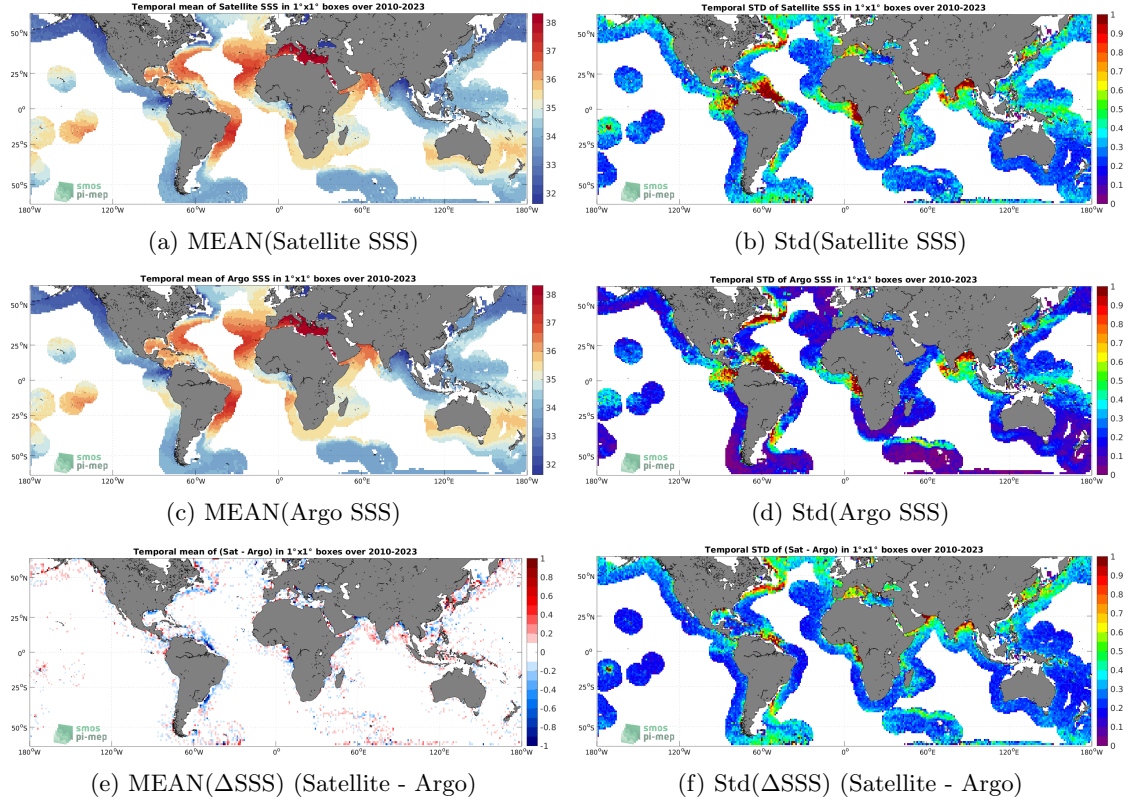
Figure 6: Temporal mean (left) and Std (right) of SSS from SMOS SSS L3 v8 - 9 Days (CATDS-CECOS-LOCEAN) (top), Argo (middle), and of \Delta SSS (Satellite - Argo). Only match-up pairs are used to generate these maps.
