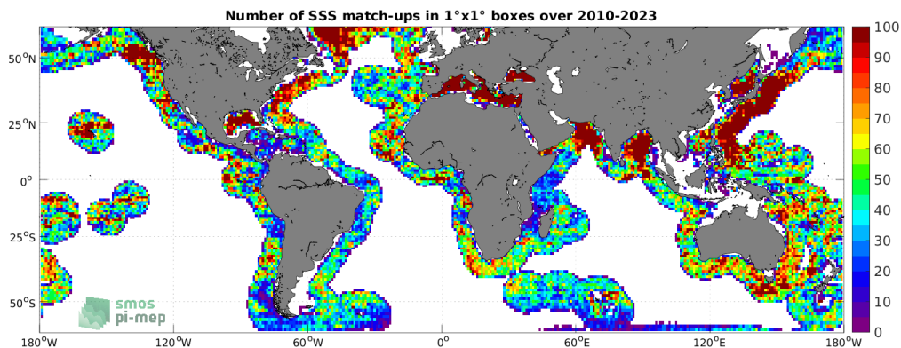
Figure 4: Number of SSS match-ups between Argo SSS and the SMOS SSS L3 v8 - 9 Days (CATDS-CECOS-LOCEAN) SSS product for the SMOS coastal zone ( <800\text{km} ) 60N-60S Pi-MEP region over 1^\circ \times 1^\circ boxes and for the full satellite product period.
