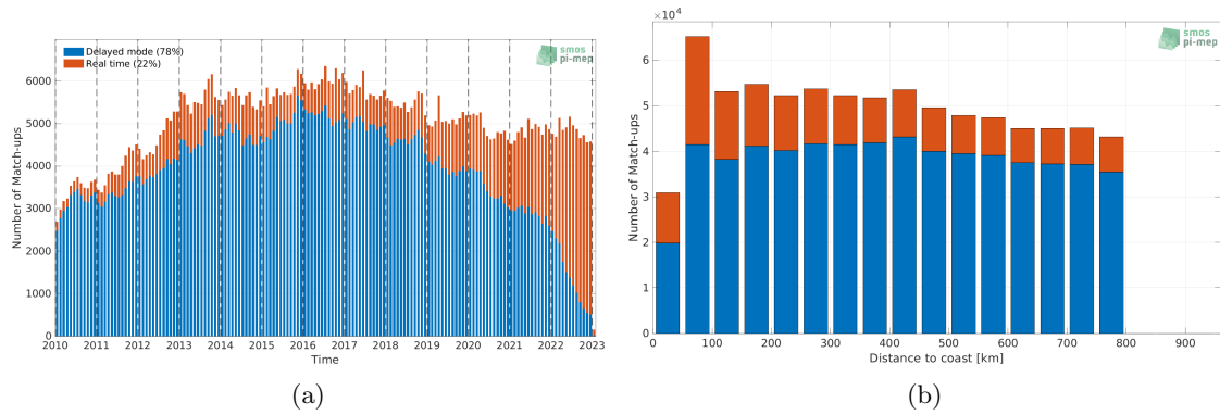
Figure 1: Number of match-ups between Argo and SMOS SSS L3 v8 - 9 Days (CATDS-CECOS-LOCEAN) SSS as a function of time (a) and as function of the distance to coast (b) over the SMOS coastal zone (<800km) 60N-60S Pi-MEP region and for the full satellite product period.
