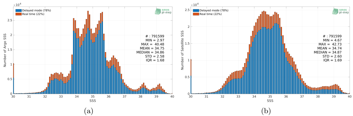
Figure 2: Histograms of SSS from Argo (a) and SMOS SSS L3 v8 - 9 Days (CATDS-CECOS-LOCEAN) (b) considering all match-up pairs per bins of 0.1 over the SMOS coastal zone (<800km) 60N-60S Pi-MEP region and for the full satellite product period.
