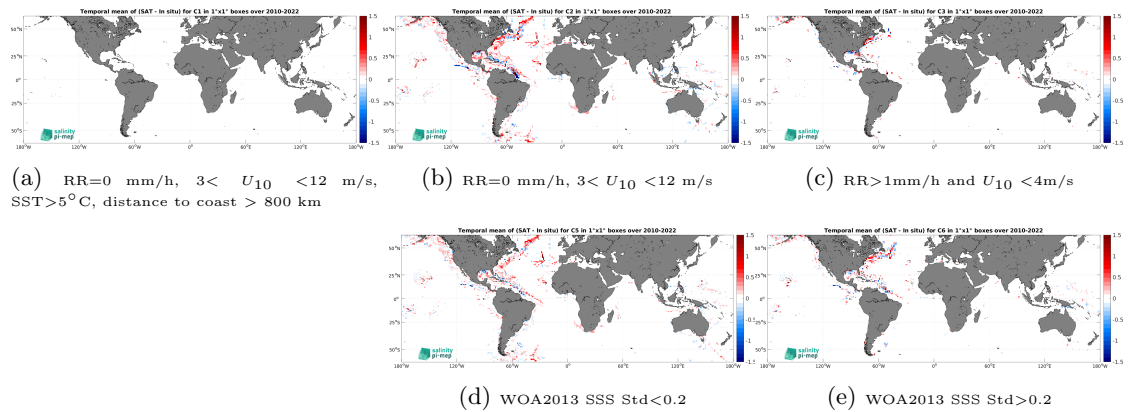
Figure 12: Temporal mean gridded over spatial boxes of size 1^\circ \times 1^\circ of \Delta SSS (SMOS SSS L3 v8 - 18 Days (CATDS-CEC-LOCEAN) - TSG (SAMOS)) for 5 different subdatasets corresponding to:RR=0 mm/h, 3 < U_{10} < 12 m/s, SST >5^\circ C, distance to coast > 800 km (a), RR=0 mm/h, 3 < U_{10} < 12 m/s (b), RR >1 mm/h and U_{10} < 4 m/s (c), WOA2013 SSS Std <0.2 (d), WOA2013 SSS Std >0.2 (e).
