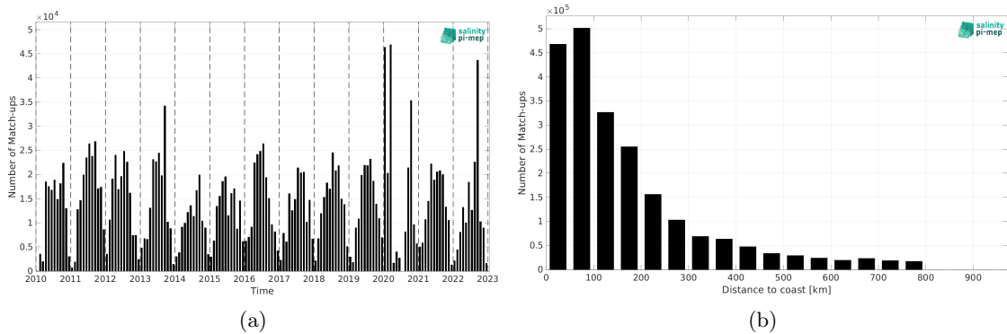
Figure 1: Number of match-ups between TSG (SAMOS) and SMOS SSS L3 v8 - 18 Days (CATDS-CEC-LOCEAN) SSS as a function of time (a) and as function of the distance to coast (b) over the SMOS coastal zone (<800km) 60N-60S Pi-MEP region and for the full satellite product period.
