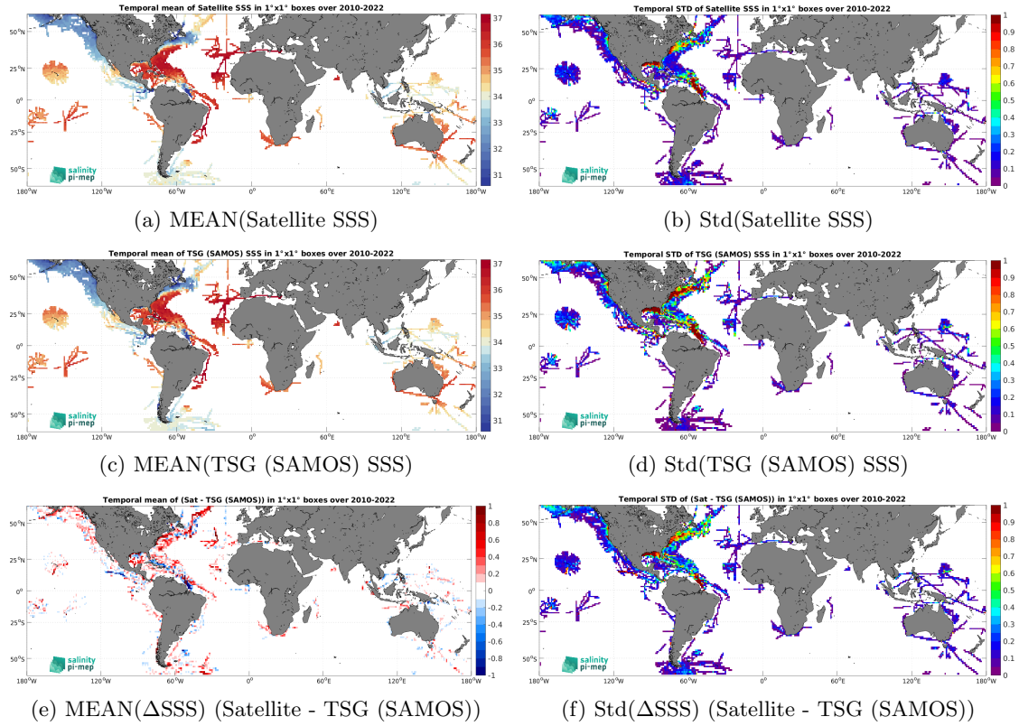
Figure 6: Temporal mean (left) and Std (right) of SSS from SMOS SSS L3 v8 - 18 Days (CATDS-CEC-LOCEAN) (top), TSG (SAMOS) (middle), and of \Delta SSS (Satellite - TSG (SAMOS)). Only match-up pairs are used to generate these maps.
