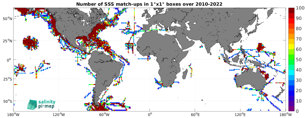
Figure 4: Number of SSS match-ups between TSG (SAMOS) SSS and the SMOS SSS L3 v8 - 18 Days (CATDS-CEC-LOCEAN) SSS product for the SMOS coastal zone (<800km) 60N-60S Pi-MEP region over 1^\circ \times 1^\circ boxes and for the full satellite product period.
