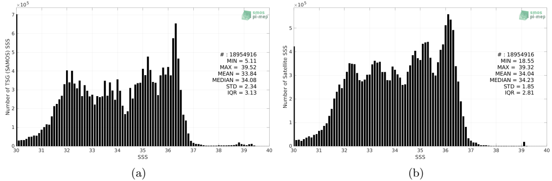
Figure 2: Histograms of SSS from TSG (SAMOS) (a) and SMOS SSS L3 v8 - 18 Days (CATDS-CECOS-LOCEAN) (b) considering all match-up pairs per bins of 0.1 over the SMOS coastal zone (<800km) 60N-60S Pi-MEP region and for the full satellite product period.
