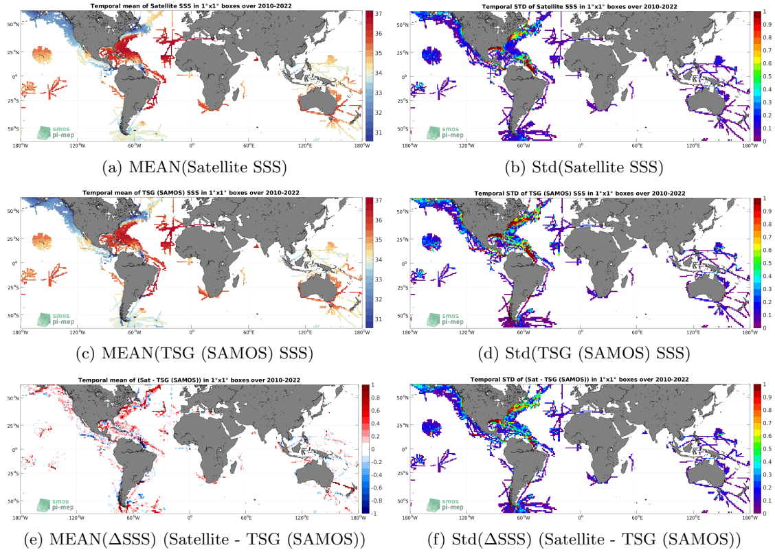
Figure 6: Temporal mean (left) and Std (right) of SSS from SMOS SSS L3 v8 - 18 Days (CATDS-CECOS-LOCEAN) (top), TSG (SAMOS) (middle), and of \Delta SSS (Satellite - TSG (SAMOS)). Only match-up pairs are used to generate these maps.
