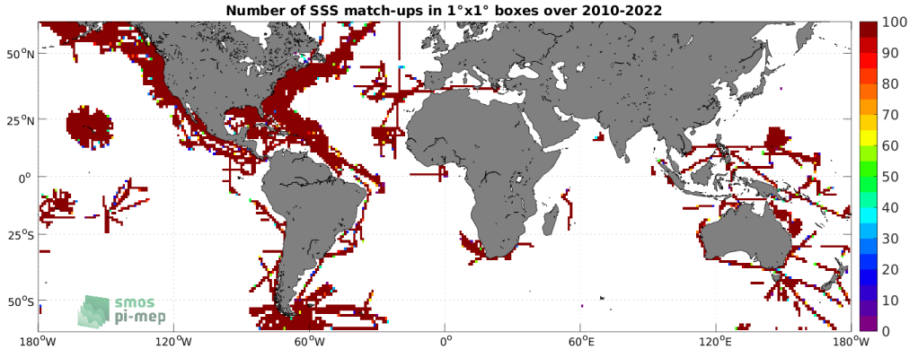
Figure 4: Number of SSS match-ups between TSG (SAMOS) SSS and the SMOS SSS L3 v8 - 18 Days (CATDS-CECOS-LOCEAN) SSS product for the SMOS coastal zone (<800km) 60N-60S Pi-MEP region over 1^\circ \times 1^\circ boxes and for the full satellite product period.
