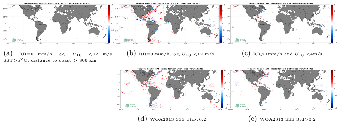
Figure 12: Temporal mean gridded over spatial boxes of size 1^\circ \times 1^\circ of \Delta\text{SSS} (SMOS SSS L3 v8 - 18 Days (CATDS-CECOS-LOCEAN) - TSG (SAMOS)) for 5 different subdatasets corresponding to:RR=0 mm/h, 3 < U_{10} < 12 m/s, SST >5^\circ\text{C} , distance to coast > 800 km (a), RR=0 mm/h, 3 < U_{10} < 12 m/s (b), RR >1 mm/h and U_{10} < 4 m/s (c), WOA2013 SSS Std <0.2 (d), WOA2013 SSS Std >0.2 (e).
