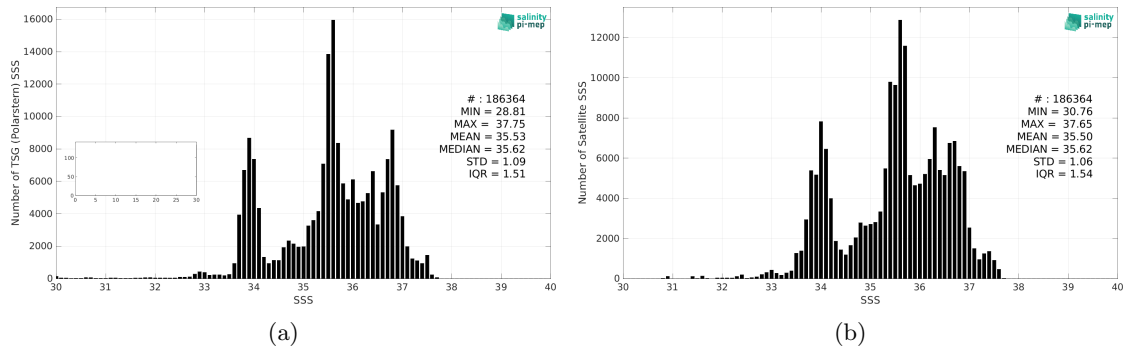
Figure 2: Histograms of SSS from TSG (Polarstern) (a) and SMOS SSS L3 v8 - 18 Days (CATDS-CEC-LOCEAN) (b) considering all match-up pairs per bins of 0.1 over the SMOS coastal zone (<800km) 60N-60S Pi-MEP region and for the full satellite product period.
