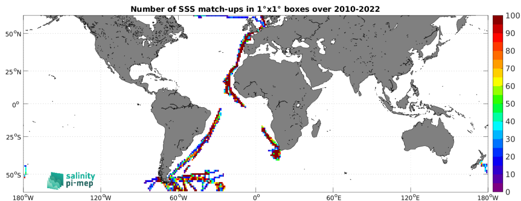
Figure 4: Number of SSS match-ups between TSG (Polarstern) SSS and the SMOS SSS L3 v8 - 18 Days (CATDS-CEC-LOCEAN) SSS product for the SMOS coastal zone (<800km) 60N-60S Pi-MEP region over 1^\circ \times 1^\circ boxes and for the full satellite product period.
