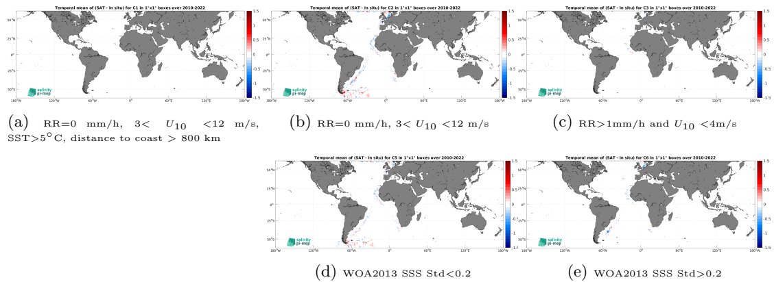
Figure 12: Temporal mean gridded over spatial boxes of size 1^\circ \times 1^\circ of \Delta SSS (SMOS SSS L3 v8 - 18 Days (CATDS-CEC-LOCEAN) - TSG (Polarstern)) for 5 different subdatasets corresponding to:RR=0 mm/h, 3 < U_{10} < 12 m/s, SST >5^\circ C, distance to coast > 800 km (a), RR=0 mm/h, 3 < U_{10} < 12 m/s (b), RR >1 mm/h and U_{10} < 4 m/s (c), WOA2013 SSS Std <0.2 (d), WOA2013 SSS Std >0.2 (e).
