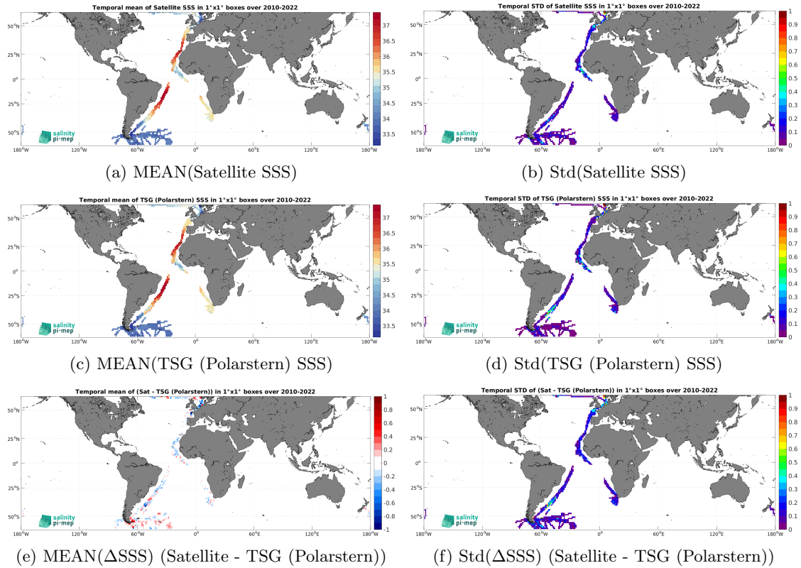
Figure 6: Temporal mean (left) and Std (right) of SSS from SMOS SSS L3 v8 - 18 Days (CATDS-CEC-LOCEAN) (top), TSG (Polarstern) (middle), and of \Delta SSS (Satellite - TSG (Polarstern)). Only match-up pairs are used to generate these maps.
