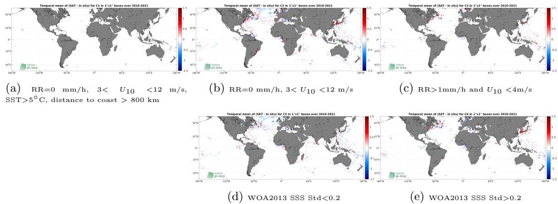
Figure 12: Temporal mean gridded over spatial boxes of size 1^\circ \times 1^\circ of \Delta\text{SSS} (SMOS SSS L3 v8 - 18 Days (CATDS-CECOS-LOCEAN) - TSG (LEGOS-DM)) for 5 different subdatasets corresponding to:RR=0 mm/h, 3 < U_{10} < 12 m/s, SST >5^\circ\text{C} , distance to coast > 800 km (a), RR=0 mm/h, 3 < U_{10} < 12 m/s (b), RR >1 mm/h and U_{10} < 4 m/s (c), WOA2013 SSS Std <0.2 (d), WOA2013 SSS Std >0.2 (e).
