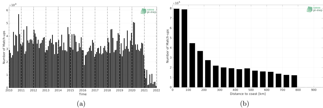
Figure 1: Number of match-ups between TSG (LEGOS-DM) and SMOS SSS L3 v8 - 18 Days (CATDS-CECOS-LOCEAN) SSS as a function of time (a) and as function of the distance to coast (b) over the SMOS coastal zone (<800km) 60N-60S Pi-MEP region and for the full satellite product period.
