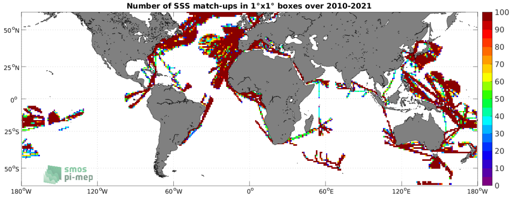
Figure 4: Number of SSS match-ups between TSG (LEGOS-DM) SSS and the SMOS SSS L3 v8 - 18 Days (CATDS-CECOS-LOCEAN) SSS product for the SMOS coastal zone (<800km) 60N-60S Pi-MEP region over 1^\circ \times 1^\circ boxes and for the full satellite product period.
