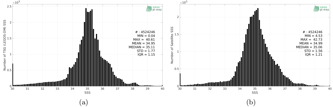
Figure 2: Histograms of SSS from TSG (LEGOS-DM) (a) and SMOS SSS L3 v8 - 18 Days (CATDS-CECOS-LOCEAN) (b) considering all match-up pairs per bins of 0.1 over the SMOS coastal zone (<800km) 60N-60S Pi-MEP region and for the full satellite product period.
