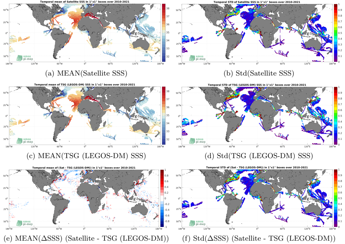
Figure 6: Temporal mean (left) and Std (right) of SSS from SMOS SSS L3 v8 - 18 Days (CATDS-CECOS-LOCEAN) (top), TSG (LEGOS-DM) (middle), and of \Delta SSS (Satellite - TSG (LEGOS-DM)). Only match-up pairs are used to generate these maps.
