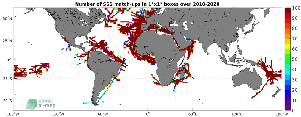
Figure 4: Number of SSS match-ups between TSG (GOSUD-Research-vessel) SSS and the SMOS SSS L3 v8 - 18 Days (CATDS-CECOS-LOCEAN) SSS product for the SMOS coastal zone (<800km) 60N-60S Pi-MEP region over 1^\circ \times 1^\circ boxes and for the full satellite product period.
