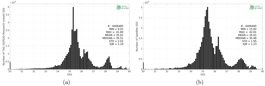
Figure 2: Histograms of SSS from TSG (GOSUD-Research-vessel) (a) and SMOS SSS L3 v8 - 18 Days (CATDS-CECOS-LOCEAN) (b) considering all match-up pairs per bins of 0.1 over the SMOS coastal zone (<800km) 60N-60S Pi-MEP region and for the full satellite product period.
