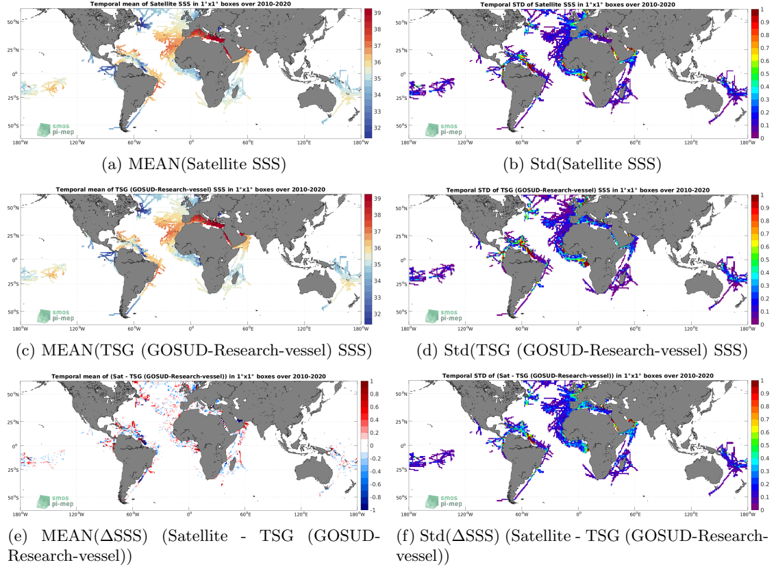
Figure 6: Temporal mean (left) and Std (right) of SSS from SMOS SSS L3 v8 - 18 Days (CATDS-CECOS-LOCEAN) (top), TSG (GOSUD-Research-vessel) (middle), and of \Delta\text{SSS} (Satellite - TSG (GOSUD-Research-vessel)). Only match-up pairs are used to generate these maps.
