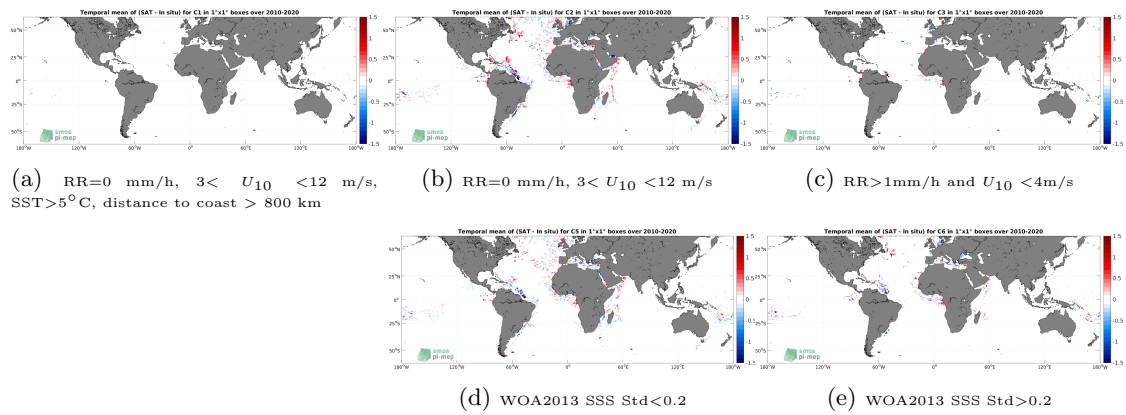
Figure 12: Temporal mean gridded over spatial boxes of size 1^\circ \times 1^\circ of \Delta SSS (SMOS SSS L3 v8 - 18 Days (CATDS-CECOS-LOCEAN) - TSG (GOSUD-Research-vessel)) for 5 different sub-datasets corresponding to:RR=0 mm/h, 3 < U_{10} < 12 m/s, SST >5^\circ C, distance to coast > 800 km (a), RR=0 mm/h, 3 < U_{10} < 12 m/s (b), RR >1 mm/h and U_{10} < 4 m/s (c), WOA2013 SSS Std <0.2 (d), WOA2013 SSS Std >0.2 (e).
