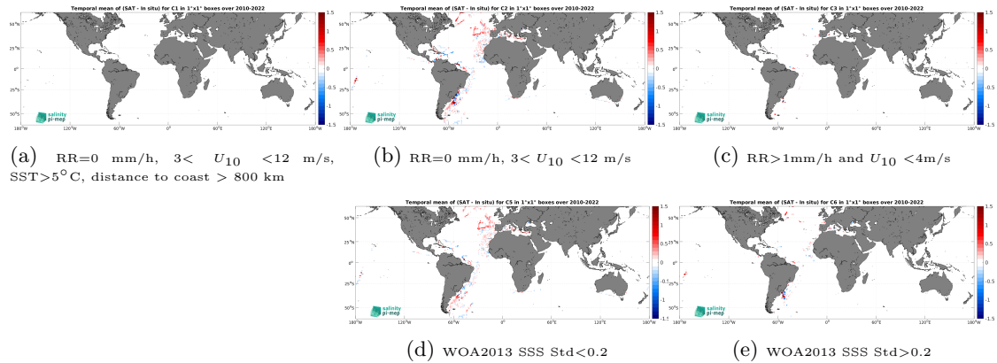
Figure 12: Temporal mean gridded over spatial boxes of size 1^\circ \times 1^\circ of \Delta SSS (SMOS SSS L3 v8 - 18 Days (CATDS-CEC-LOCEAN) - TSG (CSIC-UTM)) for 5 different subdatasets corresponding to:RR=0 mm/h, 3 < U_{10} < 12 m/s, SST >5^\circ C, distance to coast > 800 km (a), RR=0 mm/h, 3 < U_{10} < 12 m/s (b), RR >1 mm/h and U_{10} < 4 m/s (c), WOA2013 SSS Std <0.2 (d), WOA2013 SSS Std >0.2 (e).
