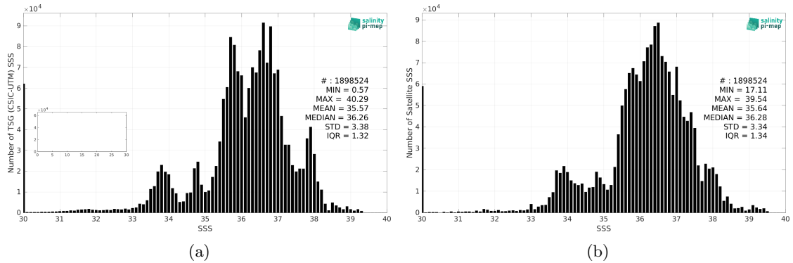
Figure 2: Histograms of SSS from TSG (CSIC-UTM) (a) and SMOS SSS L3 v8 - 18 Days (CATDS-CEC-LOCEAN) (b) considering all match-up pairs per bins of 0.1 over the SMOS coastal zone (<800km) 60N-60S Pi-MEP region and for the full satellite product period.
