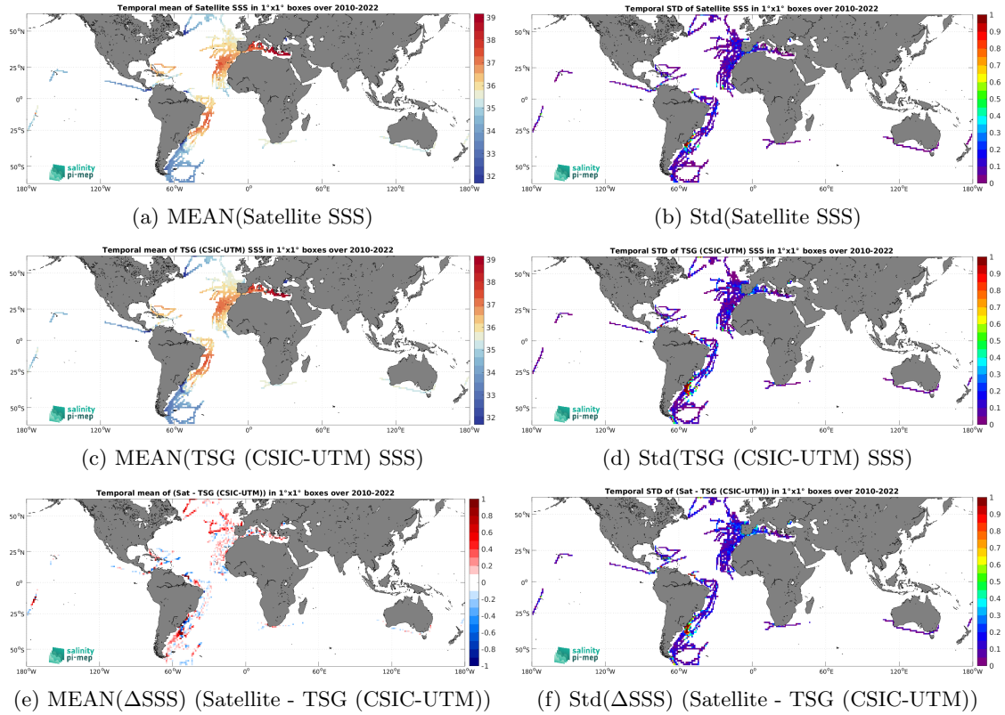
Figure 6: Temporal mean (left) and Std (right) of SSS from SMOS SSS L3 v8 - 18 Days (CATDS-CEC-LOCEAN) (top), TSG (CSIC-UTM) (middle), and of \Delta\text{SSS} (Satellite - TSG (CSIC-UTM)). Only match-up pairs are used to generate these maps.
