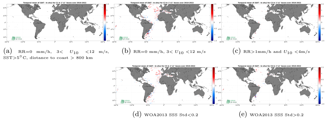
Figure 12: Temporal mean gridded over spatial boxes of size 1^\circ \times 1^\circ of \Delta\text{SSS} (SMOS SSS L3 v8 - 18 Days (CATDS-CECOS-LOCEAN) - TSG (CSIC-UTM)) for 5 different subdatasets corresponding to:RR=0 mm/h, 3 < U_{10} < 12 m/s, SST >5^\circ\text{C} , distance to coast > 800 km (a), RR=0 mm/h, 3 < U_{10} < 12 m/s (b), RR >1 mm/h and U_{10} < 4 m/s (c), WOA2013 SSS Std <0.2 (d), WOA2013 SSS Std >0.2 (e).
