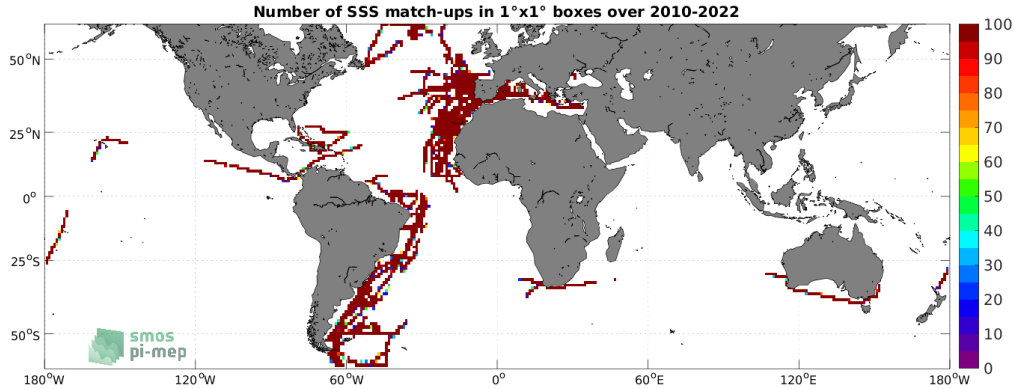
Figure 4: Number of SSS match-ups between TSG (CSIC-UTM) SSS and the SMOS SSS L3 v8 - 18 Days (CATDS-CECOS-LOCEAN) SSS product for the SMOS coastal zone ( <800\text{km} ) 60N-60S Pi-MEP region over 1^\circ \times 1^\circ boxes and for the full satellite product period.
