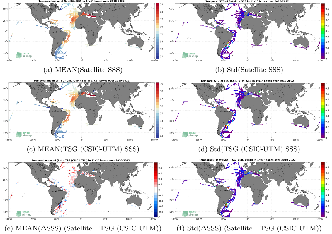
Figure 6: Temporal mean (left) and Std (right) of SSS from SMOS SSS L3 v8 - 18 Days (CATDS-CECOS-LOCEAN) (top), TSG (CSIC-UTM) (middle), and of \Delta\text{SSS} (Satellite - TSG (CSIC-UTM)). Only match-up pairs are used to generate these maps.
