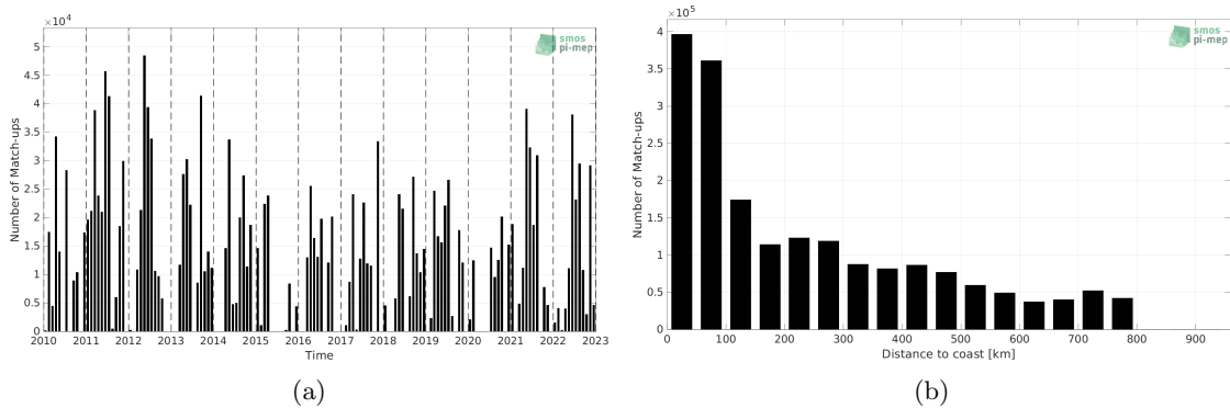
Figure 1: Number of match-ups between TSG (CSIC-UTM) and SMOS SSS L3 v8 - 18 Days (CATDS-CECOS-LOCEAN) SSS as a function of time (a) and as function of the distance to coast (b) over the SMOS coastal zone (<800km) 60N-60S Pi-MEP region and for the full satellite product period.
