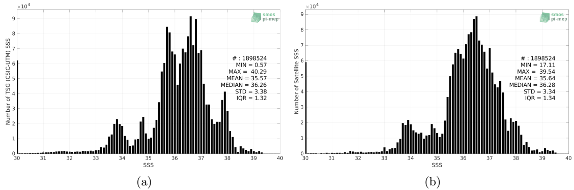
Figure 2: Histograms of SSS from TSG (CSIC-UTM) (a) and SMOS SSS L3 v8 - 18 Days (CATDS-CECOS-LOCEAN) (b) considering all match-up pairs per bins of 0.1 over the SMOS coastal zone (<800km) 60N-60S Pi-MEP region and for the full satellite product period.
