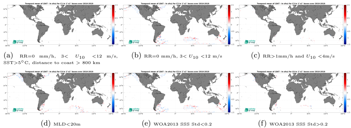
Figure 12: Temporal mean gridded over spatial boxes of size 1^{\circ}\times 1^{\circ} of \Delta\text{SSS} (SMOS SSS L3 v8 - 18 Days (CATDS-CEC-LOCEAN) - Marine mammals) for 6 different subdatasets corresponding to:RR=0 mm/h, 3 < U_{10} < 12 m/s, SST >5^{\circ}\text{C} , distance to coast > 800 km (a), RR=0 mm/h, 3 < U_{10} < 12 m/s (b), RR >1\text{mm/h} and U_{10} < 4\text{m/s} (c),MLD <20\text{m} (d),WOA2013 SSS Std <0.2 (e),WOA2013 SSS Std >0.2 (f).
