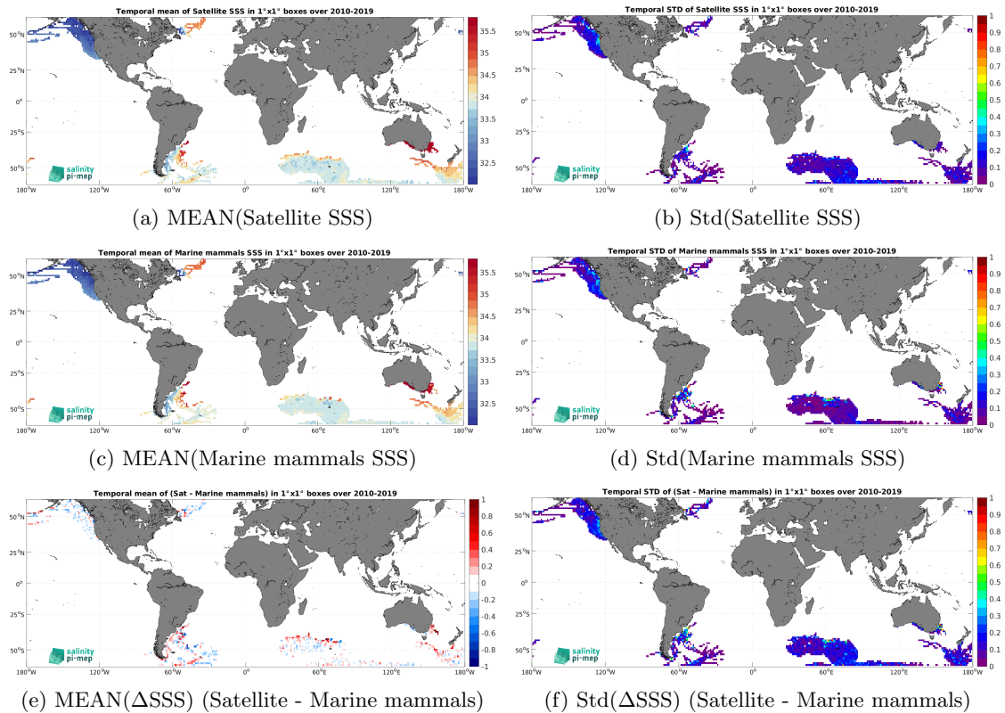
Figure 6: Temporal mean (left) and Std (right) of SSS from SMOS SSS L3 v8 - 18 Days (CATDS-CEC-LOCEAN) (top), Marine mammals (middle), and of \Delta SSS (Satellite - Marine mammals). Only match-up pairs are used to generate these maps.
