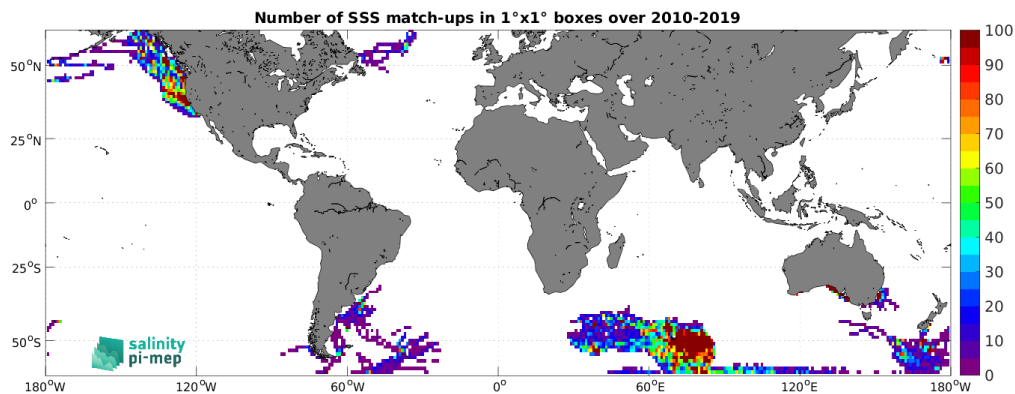
Figure 4: Number of SSS match-ups between Marine mammals SSS and the SMOS SSS L3 v8 - 18 Days (CATDS-CEC-LOCEAN) SSS product for the SMOS coastal zone (<800km) 60N-60S Pi-MEP region over 1^\circ \times 1^\circ boxes and for the full satellite product period.
