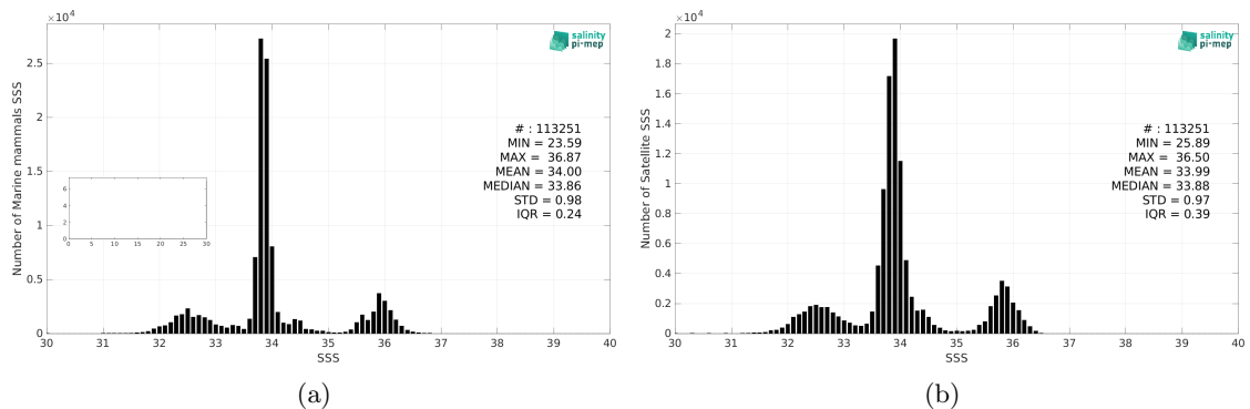
Figure 2: Histograms of SSS from Marine mammals (a) and SMOS SSS L3 v8 - 18 Days (CATDS-CEC-LOCEAN) (b) considering all match-up pairs per bins of 0.1 over the SMOS coastal zone (<800km) 60N-60S Pi-MEP region and for the full satellite product period.
