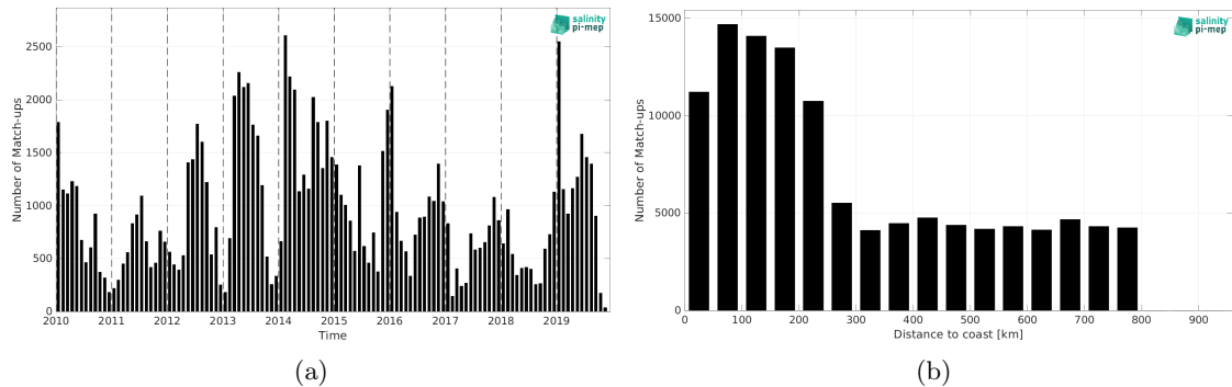
Figure 1: Number of match-ups between Marine mammals and SMOS SSS L3 v8 - 18 Days (CATDS-CEC-LOCEAN) SSS as a function of time (a) and as function of the distance to coast (b) over the SMOS coastal zone (<800km) 60N-60S Pi-MEP region and for the full satellite product period.
