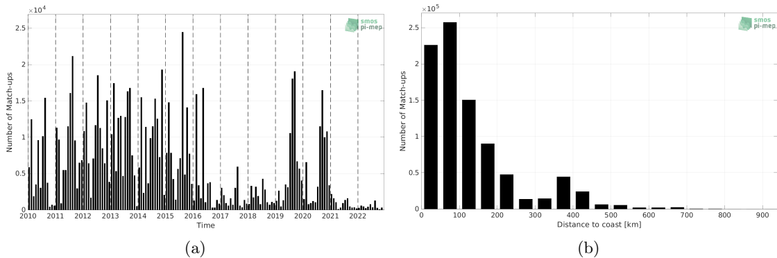
Figure 1: Number of match-ups between ICES and SMOS SSS L3 v8 - 18 Days (CATDS-CECOS-LOCEAN) SSS as a function of time (a) and as function of the distance to coast (b) over the SMOS coastal zone (<800km) 60N-60S Pi-MEP region and for the full satellite product period.
