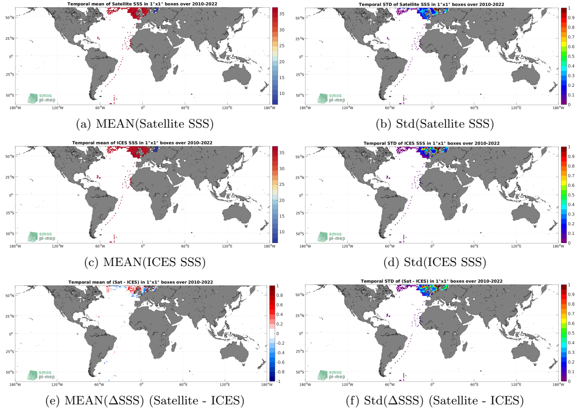
Figure 6: Temporal mean (left) and Std (right) of SSS from SMOS SSS L3 v8 - 18 Days (CATDS-CECOS-LOCEAN) (top), ICES (middle), and of \Delta SSS (Satellite - ICES). Only match-up pairs are used to generate these maps.
