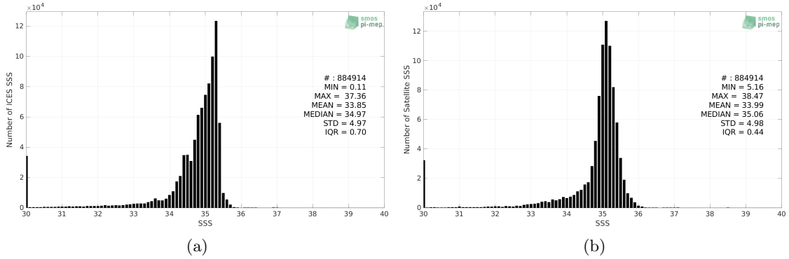
Figure 2: Histograms of SSS from ICES (a) and SMOS SSS L3 v8 - 18 Days (CATDS-CECOS-LOCEAN) (b) considering all match-up pairs per bins of 0.1 over the SMOS coastal zone (<800km) 60N-60S Pi-MEP region and for the full satellite product period.
