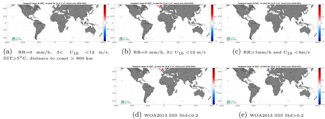
Figure 12: Temporal mean gridded over spatial boxes of size 1^\circ \times 1^\circ of \Delta SSS (SMOS SSS L3 v8 - 18 Days (CATDS-CECOS-LOCEAN) - ICES) for 5 different subdatasets corresponding to:RR=0 mm/h, 3 < U_{10} < 12 m/s, SST >5^\circ C, distance to coast > 800 km (a), RR=0 mm/h, 3 < U_{10} < 12 m/s (b), RR >1 mm/h and U_{10} < 4 m/s (c), WOA2013 SSS Std <0.2 (d), WOA2013 SSS Std >0.2 (e).
