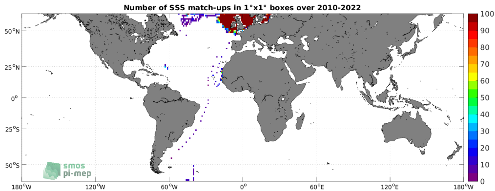
Figure 4: Number of SSS match-ups between ICES SSS and the SMOS SSS L3 v8 - 18 Days (CATDS-CECOS-LOCEAN) SSS product for the SMOS coastal zone ( <800\text{km} ) 60N-60S Pi-MEP region over 1^\circ \times 1^\circ boxes and for the full satellite product period.
