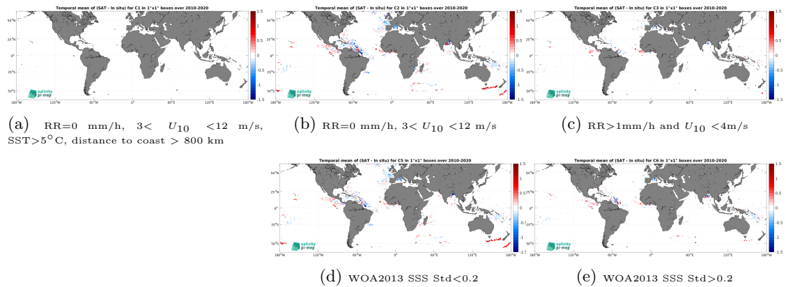
Figure 11: Temporal mean gridded over spatial boxes of size 1^\circ \times 1^\circ of \Delta\text{SSS} (SMOS SSS L3 v8 - 18 Days (CATDS-CEC-LOCEAN) - Surface drifters) for 5 different subdatasets corresponding to:RR=0 mm/h, 3 < U_{10} < 12 m/s, SST >5^\circ\text{C} , distance to coast > 800 km (a), RR=0 mm/h, 3 < U_{10} < 12 m/s (b), RR >1 mm/h and U_{10} < 4 m/s (c), WOA2013 SSS Std <0.2 (d), WOA2013 SSS Std >0.2 (e).
