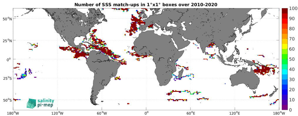
Figure 3: Number of SSS match-ups between Surface drifters SSS and the SMOS SSS L3 v8 - 18 Days (CATDS-CEC-LOCEAN) SSS product for the SMOS coastal zone (<800km) 60N-60S Pi-MEP region over 1^\circ \times 1^\circ boxes and for the full satellite product period.
