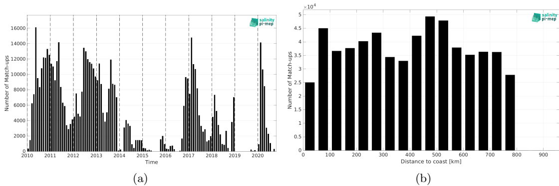
Figure 1: Number of match-ups between Surface drifters and SMOS SSS L3 v8 - 18 Days (CATDS-CEC-LOCEAN) SSS as a function of time (a) and as function of the distance to coast (b) over the SMOS coastal zone (<800km) 60N-60S Pi-MEP region and for the full satellite product period.
