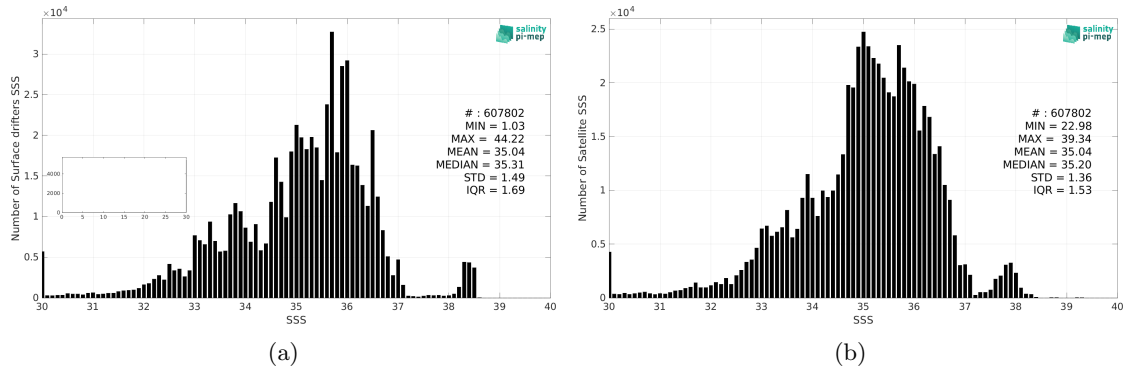
Figure 2: Histograms of SSS from Surface drifters (a) and SMOS SSS L3 v8 - 18 Days (CATDS-CEC-LOCEAN) (b) considering all match-up pairs per bins of 0.1 over the SMOS coastal zone (<800km) 60N-60S Pi-MEP region and for the full satellite product period.
