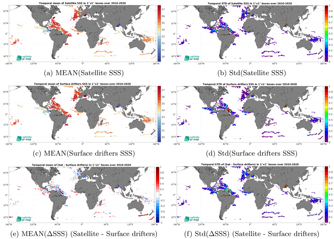
Figure 5: Temporal mean (left) and Std (right) of SSS from SMOS SSS L3 v8 - 18 Days (CATDS-CEC-LOCEAN) (top), Surface drifters (middle), and of \Delta SSS (Satellite - Surface drifters). Only match-up pairs are used to generate these maps.
