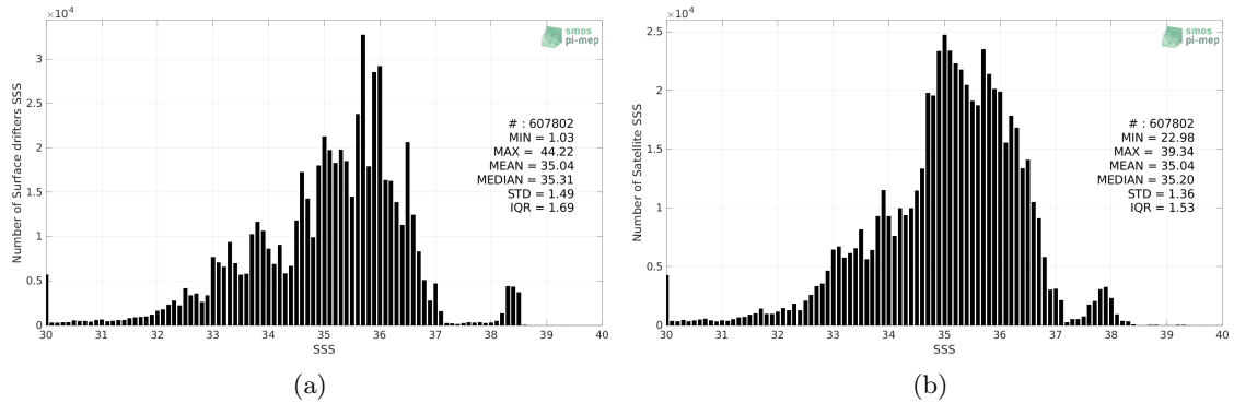
Figure 2: Histograms of SSS from Surface drifters (a) and SMOS SSS L3 v8 - 18 Days (CATDS-CECOS-LOCEAN) (b) considering all match-up pairs per bins of 0.1 over the SMOS coastal zone (<800km) 60N-60S Pi-MEP region and for the full satellite product period.
