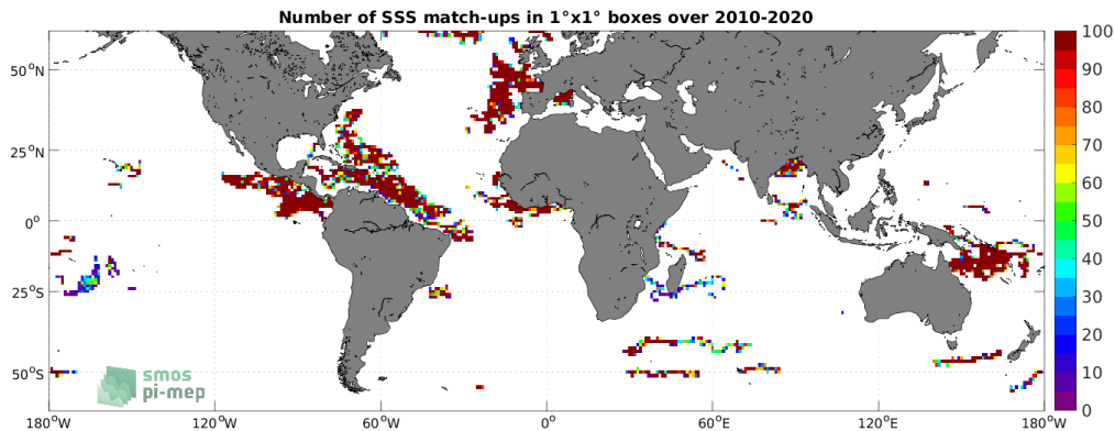
Figure 3: Number of SSS match-ups between Surface drifters SSS and the SMOS SSS L3 v8 - 18 Days (CATDS-CECOS-LOCEAN) SSS product for the SMOS coastal zone (<800km) 60N-60S Pi-MEP region over 1^\circ \times 1^\circ boxes and for the full satellite product period.
