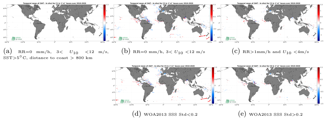
Figure 11: Temporal mean gridded over spatial boxes of size 1^\circ \times 1^\circ of \Delta SSS (SMOS SSS L3 v8 - 18 Days (CATDS-CECOS-LOCEAN) - Surface drifters) for 5 different subdatasets corresponding to:RR=0 mm/h, 3 < U_{10} < 12 m/s, SST >5^\circ C, distance to coast > 800 km (a), RR=0 mm/h, 3 < U_{10} < 12 m/s (b), RR >1 mm/h and U_{10} < 4 m/s (c), WOA2013 SSS Std <0.2 (d), WOA2013 SSS Std >0.2 (e).
