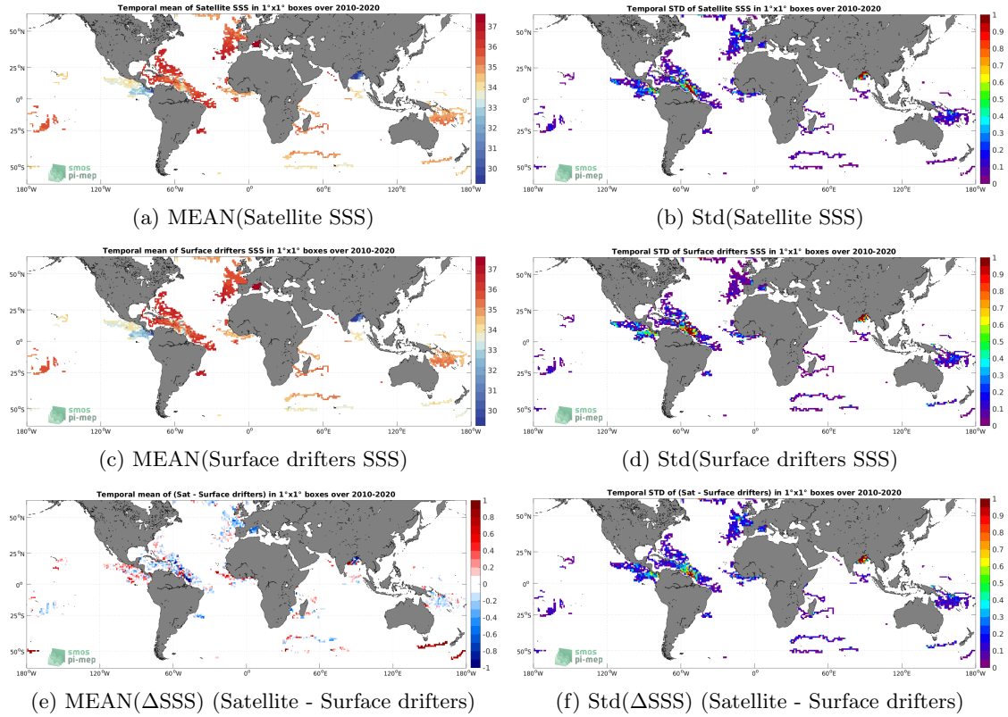
Figure 5: Temporal mean (left) and Std (right) of SSS from SMOS SSS L3 v8 - 18 Days (CATDS-CECOS-LOCEAN) (top), Surface drifters (middle), and of \Delta SSS (Satellite - Surface drifters). Only match-up pairs are used to generate these maps.
