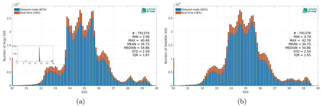
Figure 2: Histograms of SSS from Argo (a) and SMOS SSS L3 v8 - 18 Days (CATDS-CEC-LOCEAN) (b) considering all match-up pairs per bins of 0.1 over the SMOS coastal zone (<800km) 60N-60S Pi-MEP region and for the full satellite product period.
