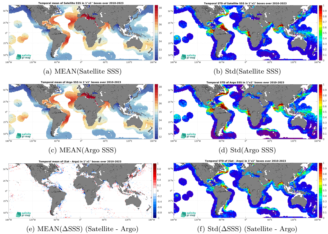
Figure 6: Temporal mean (left) and Std (right) of SSS from SMOS SSS L3 v8 - 18 Days (CATDS-CEC-LOCEAN) (top), Argo (middle), and of \Delta SSS (Satellite - Argo). Only match-up pairs are used to generate these maps.
