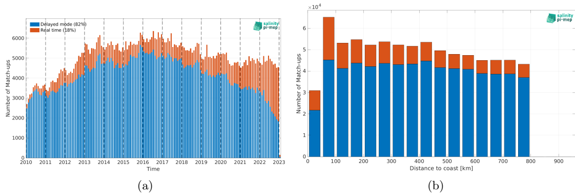
Figure 1: Number of match-ups between Argo and SMOS SSS L3 v8 - 18 Days (CATDS-CEC-LOCEAN) SSS as a function of time (a) and as function of the distance to coast (b) over the SMOS coastal zone (<800km) 60N-60S Pi-MEP region and for the full satellite product period.
