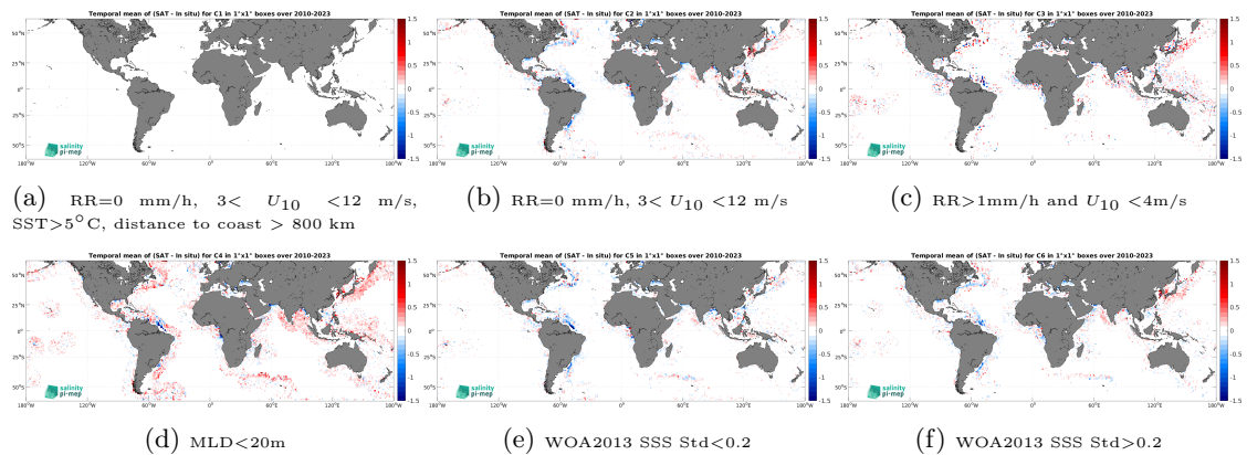
Figure 12: Temporal mean gridded over spatial boxes of size 1^\circ \times 1^\circ of \Delta SSS (SMOS SSS L3 v8 - 18 Days (CATDS-CEC-LOCEAN) - Argo) for 6 different subdatasets corresponding to:RR=0 mm/h, 3 < U_{10} < 12 m/s, SST >5^\circ C, distance to coast > 800 km (a), RR=0 mm/h, 3 < U_{10} < 12 m/s (b), RR >1 mm/h and U_{10} < 4 m/s (c),MLD <20 m (d),WOA2013 SSS Std <0.2 (e),WOA2013 SSS Std >0.2 (f).
