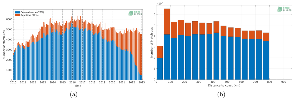
Figure 1: Number of match-ups between Argo and SMOS SSS L3 v8 - 18 Days (CATDS-CECOS-LOCEAN) SSS as a function of time (a) and as function of the distance to coast (b) over the SMOS coastal zone (<800km) 60N-60S Pi-MEP region and for the full satellite product period.
