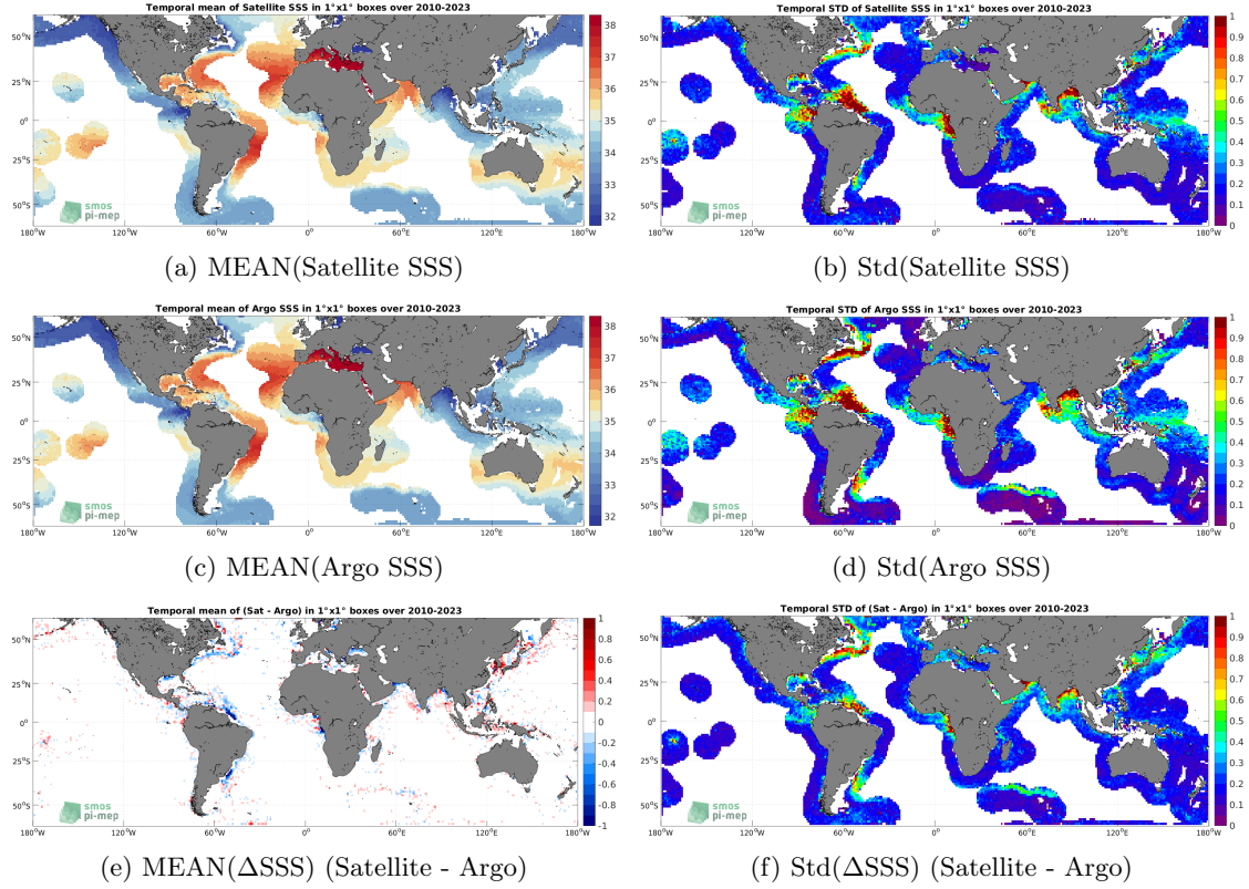
Figure 6: Temporal mean (left) and Std (right) of SSS from SMOS SSS L3 v8 - 18 Days (CATDS-CECOS-LOCEAN) (top), Argo (middle), and of \Delta SSS (Satellite - Argo). Only match-up pairs are used to generate these maps.
