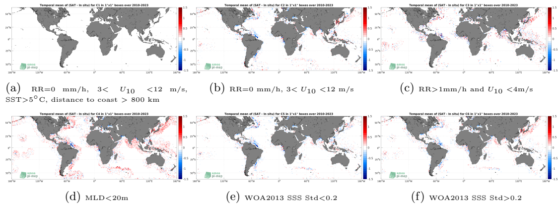
Figure 12: Temporal mean gridded over spatial boxes of size 1^\circ \times 1^\circ of \Delta SSS (SMOS SSS L3 v8 - 18 Days (CATDS-CECOS-LOCEAN) - Argo) for 6 different subdatasets corresponding to:RR=0 mm/h, 3 < U_{10} < 12 m/s, SST >5^\circ C, distance to coast > 800 km (a), RR=0 mm/h, 3 < U_{10} < 12 m/s (b), RR >1 mm/h and U_{10} < 4 m/s (c),MLD <20 m (d),WOA2013 SSS Std <0.2 (e),WOA2013 SSS Std >0.2 (f).
