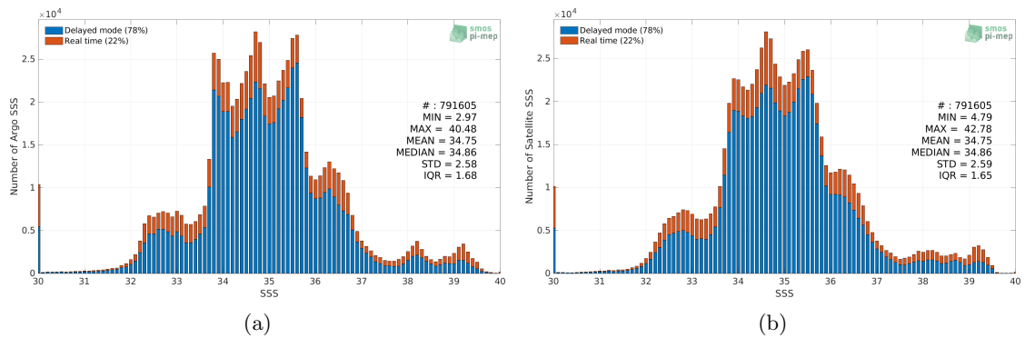
Figure 2: Histograms of SSS from Argo (a) and SMOS SSS L3 v8 - 18 Days (CATDS-CECOS-LOCEAN) (b) considering all match-up pairs per bins of 0.1 over the SMOS coastal zone (<800km) 60N-60S Pi-MEP region and for the full satellite product period.
