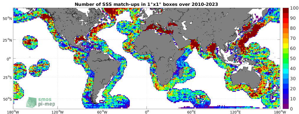
Figure 4: Number of SSS match-ups between Argo SSS and the SMOS SSS L3 v8 - 18 Days (CATDS-CECOS-LOCEAN) SSS product for the SMOS coastal zone ( <800\text{km} ) 60N-60S Pi-MEP region over 1^\circ \times 1^\circ boxes and for the full satellite product period.
