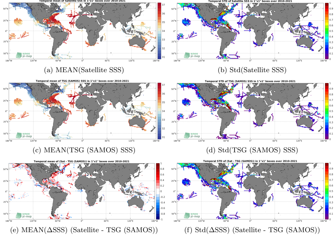
Figure 6: Temporal mean (left) and Std (right) of SSS from SMOS SSS L3 v7 - 9 Days (CATDS-CECOS-LOCEAN) (top), TSG (SAMOS) (middle), and of \Delta SSS (Satellite - TSG (SAMOS)). Only match-up pairs are used to generate these maps.
