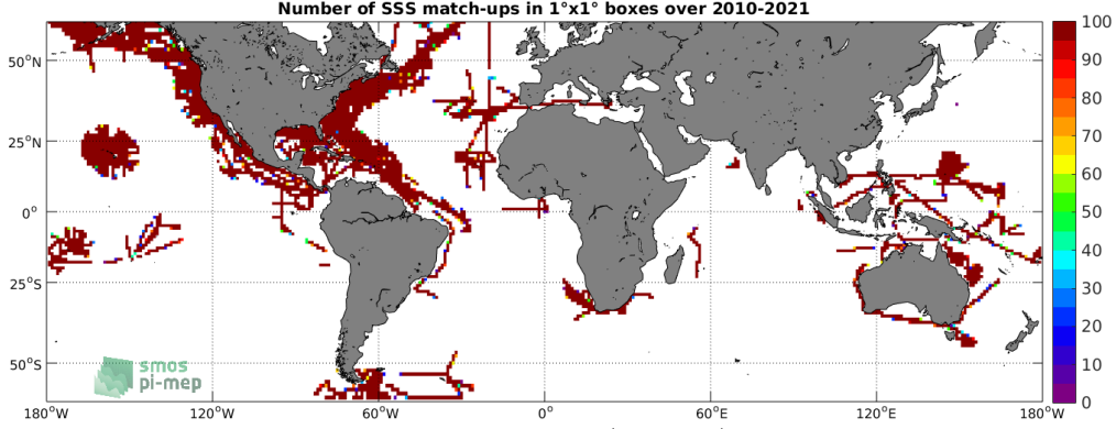
Figure 4: Number of SSS match-ups between TSG (SAMOS) SSS and the SMOS SSS L3 v7 - 9 Days (CATDS-CECOS-LOCEAN) SSS product for the SMOS coastal zone (<800km) 60N-60S Pi-MEP region over 1^\circ \times 1^\circ boxes and for the full satellite product period.
