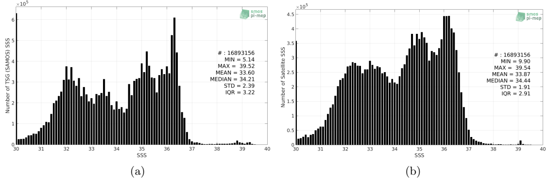
Figure 2: Histograms of SSS from TSG (SAMOS) (a) and SMOS SSS L3 v7 - 9 Days (CATDS-CECOS-LOCEAN) (b) considering all match-up pairs per bins of 0.1 over the SMOS coastal zone (<800km) 60N-60S Pi-MEP region and for the full satellite product period.
