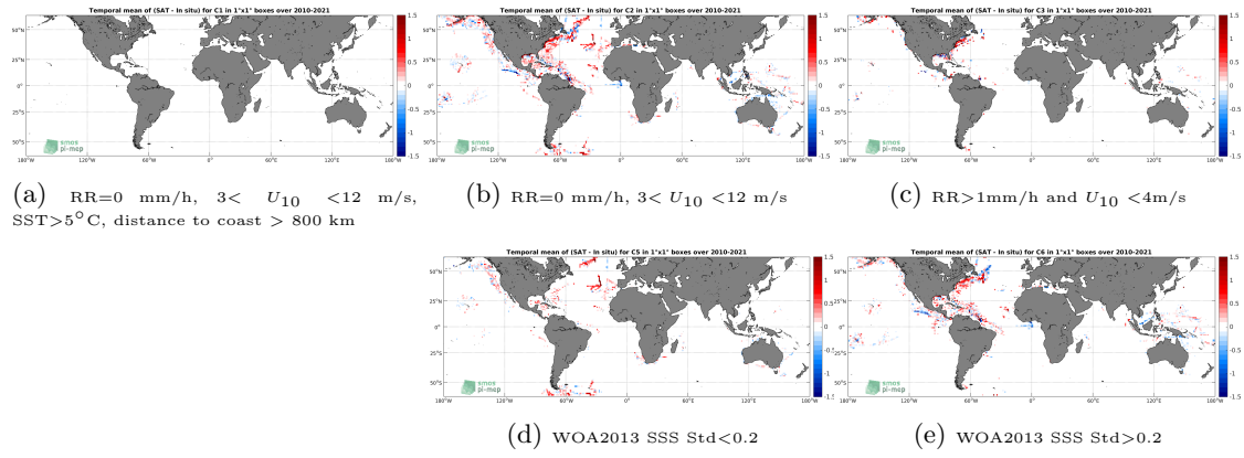
Figure 12: Temporal mean gridded over spatial boxes of size 1^\circ \times 1^\circ of \Delta SSS (SMOS SSS L3 v7 - 9 Days (CATDS-CECOS-LOCEAN) - TSG (SAMOS)) for 5 different subdatasets corresponding to: RR=0 mm/h, 3 < U_{10} < 12 m/s, SST > 5^\circ C , distance to coast > 800 km (a), RR=0 mm/h, 3 < U_{10} < 12 m/s (b), RR > 1 mm/h and U_{10} < 4 m/s (c), WOA2013 SSS Std < 0.2 (d), WOA2013 SSS Std > 0.2 (e).
