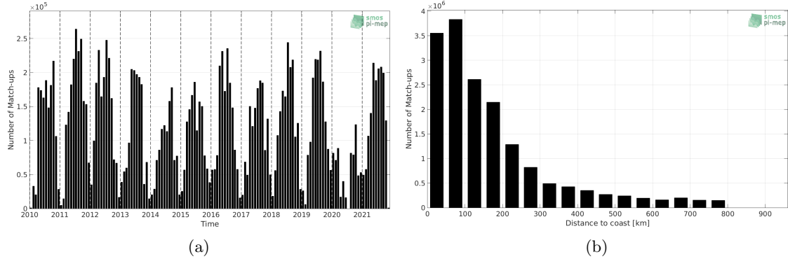
Figure 1: Number of match-ups between TSG (SAMOS) and SMOS SSS L3 v7 - 9 Days (CATDS-CECOS-LOCEAN) SSS as a function of time (a) and as function of the distance to coast (b) over the SMOS coastal zone (<800km) 60N-60S Pi-MEP region and for the full satellite product period.
