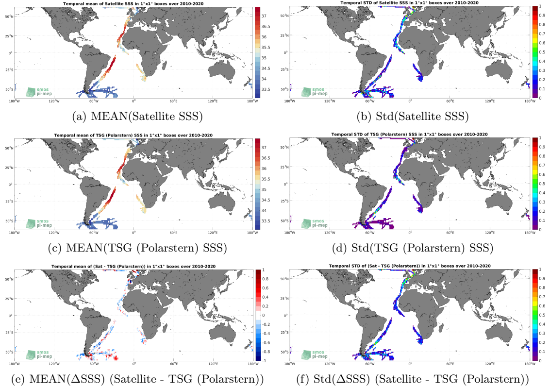
Figure 6: Temporal mean (left) and Std (right) of SSS from SMOS SSS L3 v7 - 9 Days (CATDS-CECOS-LOCEAN) (top), TSG (Polarstern) (middle), and of \Delta SSS (Satellite - TSG (Polarstern)). Only match-up pairs are used to generate these maps.
