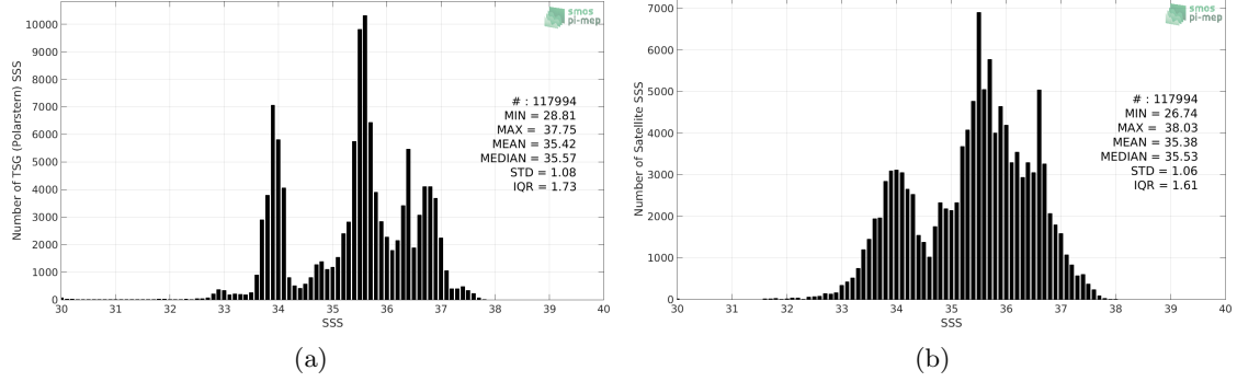
Figure 2: Histograms of SSS from TSG (Polarstern) (a) and SMOS SSS L3 v7 - 9 Days (CATDS-CECOS-LOCEAN) (b) considering all match-up pairs per bins of 0.1 over the SMOS coastal zone (<800km) 60N-60S Pi-MEP region and for the full satellite product period.
