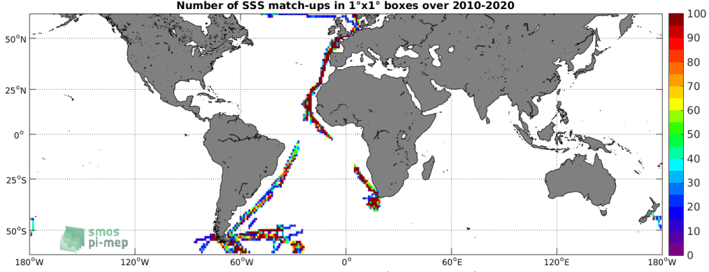
Figure 4: Number of SSS match-ups between TSG (Polarstern) SSS and the SMOS SSS L3 v7 - 9 Days (CATDS-CECOS-LOCEAN) SSS product for the SMOS coastal zone (<800km) 60N-60S Pi-MEP region over 1^\circ \times 1^\circ boxes and for the full satellite product period.
