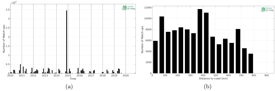
Figure 1: Number of match-ups between TSG (Polarstern) and SMOS SSS L3 v7 - 9 Days (CATDS-CECOS-LOCEAN) SSS as a function of time (a) and as function of the distance to coast (b) over the SMOS coastal zone (<800km) 60N-60S Pi-MEP region and for the full satellite product period.
