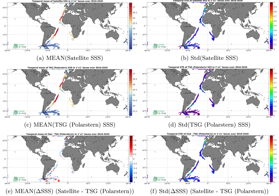
Figure 6: Temporal mean (left) and Std (right) of SSS from SMOS SSS L3 v7 - 9 Days (CATDS-CECOS-LOCEAN) (top), TSG (Polarstern) (middle), and of \Delta\text{SSS} (Satellite - TSG (Polarstern)). Only match-up pairs are used to generate these maps.
