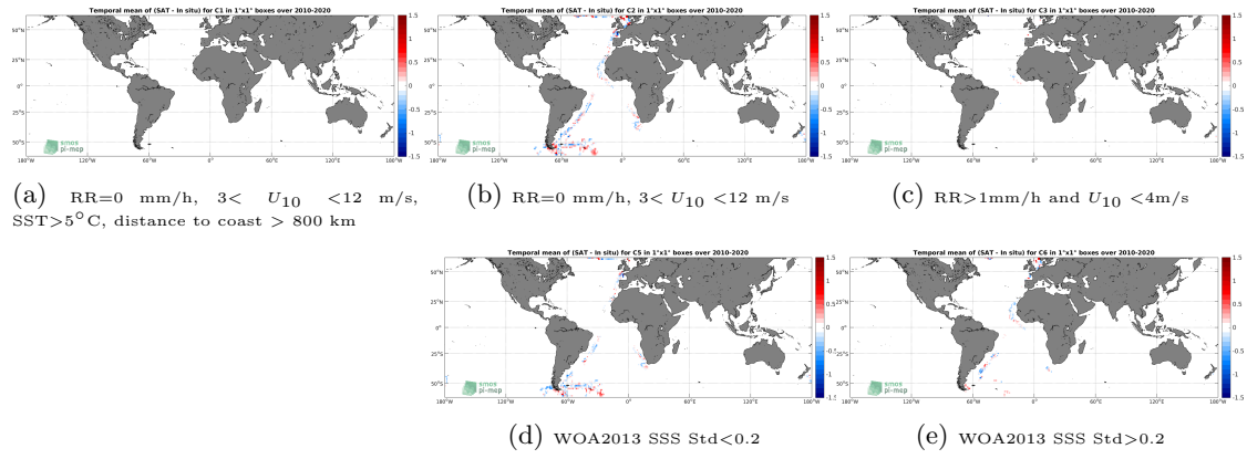
Figure 12: Temporal mean gridded over spatial boxes of size 1^\circ \times 1^\circ of \Delta SSS (SMOS SSS L3 v7 - 9 Days (CATDS-CECOS-LOCEAN) - TSG (Polarstern)) for 5 different subdatasets corresponding to: RR=0 mm/h, 3 < U_{10} < 12 m/s, SST > 5^\circ C , distance to coast > 800 km (a), RR=0 mm/h, 3 < U_{10} < 12 m/s (b), RR > 1 mm/h and U_{10} < 4 m/s (c), WOA2013 SSS Std < 0.2 (d), WOA2013 SSS Std > 0.2 (e).
