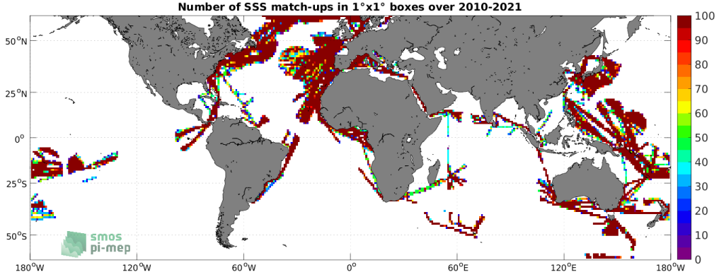
Figure 4: Number of SSS match-ups between TSG (LEGOS-DM) SSS and the SMOS SSS L3 v7 - 9 Days (CATDS-CECOS-LOCEAN) SSS product for the SMOS coastal zone (<800km) 60N-60S Pi-MEP region over 1^{\circ} \times 1^{\circ} boxes and for the full satellite product period.
