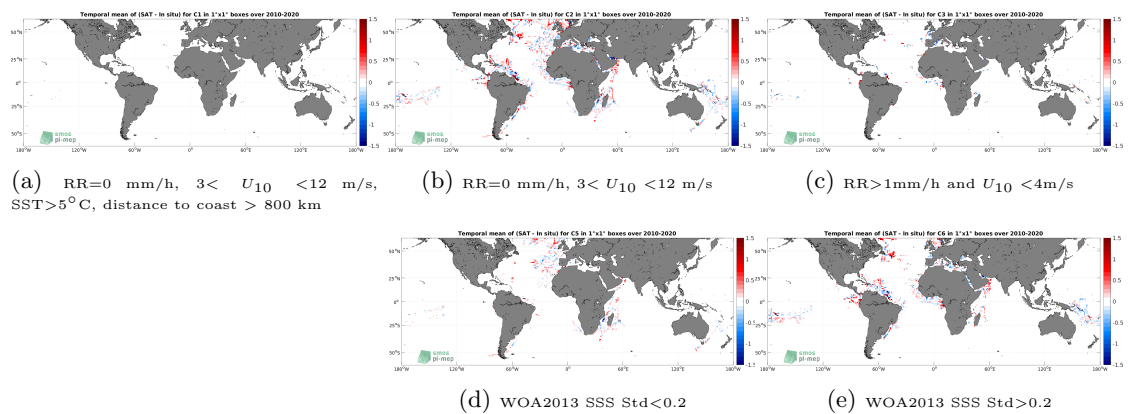
Figure 12: Temporal mean gridded over spatial boxes of size 1^\circ \times 1^\circ of \Delta SSS (SMOS SSS L3 v7 - 9 Days (CATDS-CECOS-LOCEAN) - TSG (GOSUD-Research-vessel)) for 5 different subdatasets corresponding to:RR=0 mm/h, 3 < U_{10} < 12 m/s, SST >5^\circ\text{C} , distance to coast > 800 km (a), RR=0 mm/h, 3 < U_{10} < 12 m/s (b), RR >1 mm/h and U_{10} < 4 m/s (c), WOA2013 SSS Std <0.2 (d), WOA2013 SSS Std >0.2 (e).
