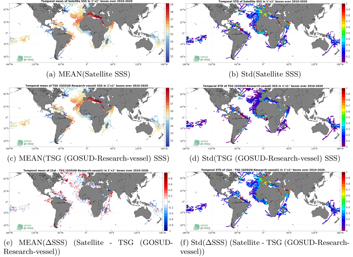
Figure 6: Temporal mean (left) and Std (right) of SSS from SMOS SSS L3 v7 - 9 Days (CATDS-CECOS-LOCEAN) (top), TSG (GOSUD-Research-vessel) (middle), and of \Delta SSS (Satellite - TSG (GOSUD-Research-vessel)). Only match-up pairs are used to generate these maps.
