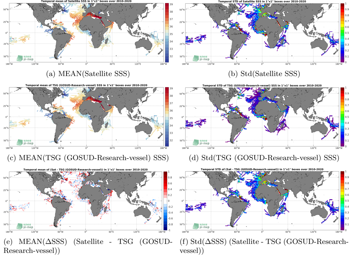
Figure 6: Temporal mean (left) and Std (right) of SSS from SMOS SSS L3 v7 - 9 Days (CATDS-CECOS-LOCEAN) (top), TSG (GOSUD-Research-vessel) (middle), and of \Delta\text{SSS} (Satellite - TSG (GOSUD-Research-vessel)). Only match-up pairs are used to generate these maps.
