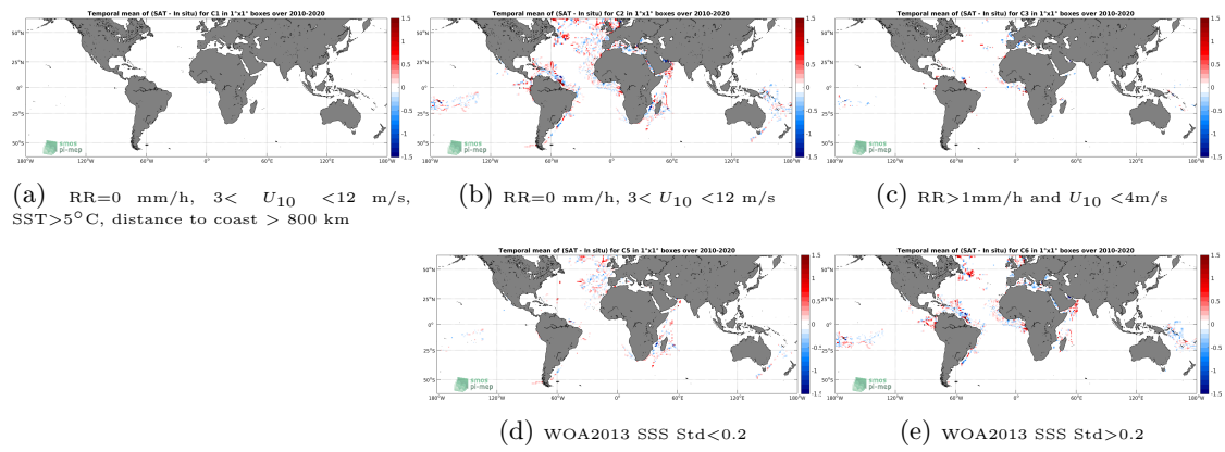
Figure 12: Temporal mean gridded over spatial boxes of size 1^\circ \times 1^\circ of \Delta\text{SSS} (SMOS SSS L3 v7 - 9 Days (CATDS-CECOS-LOCEAN) - TSG (GOSUD-Research-vessel)) for 5 different subdatasets corresponding to:RR=0 mm/h, 3 < U_{10} < 12 m/s, SST>5°C, distance to coast > 800 km (a), RR=0 mm/h, 3 < U_{10} < 12 m/s (b), RR>1mm/h and U_{10} < 4 m/s (c), WOA2013 SSS Std<0.2 (d), WOA2013 SSS Std>0.2 (e).
