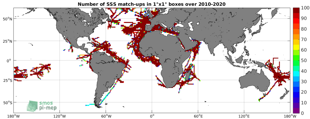
Figure 4: Number of SSS match-ups between TSG (GOSUD-Research-vessel) SSS and the SMOS SSS L3 v7 - 9 Days (CATDS-CECOS-LOCEAN) SSS product for the SMOS coastal zone (<800km) 60N-60S Pi-MEP region over 1^{\circ} \times 1^{\circ} boxes and for the full satellite product period.
