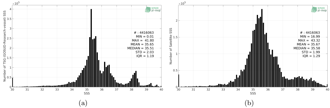
Figure 2: Histograms of SSS from TSG (GOSUD-Research-vessel) (a) and SMOS SSS L3 v7 - 9 Days (CATDS-CECOS-LOCEAN) (b) considering all match-up pairs per bins of 0.1 over the SMOS coastal zone (<800km) 60N-60S Pi-MEP region and for the full satellite product period.
