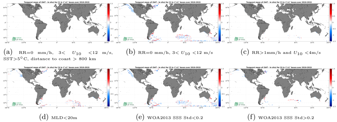
Figure 12: Temporal mean gridded over spatial boxes of size 1^{\circ}\times 1^{\circ} of \Delta\text{SSS} (SMOS SSS L3 v7 - 9 Days (CATDS-CECOS-LOCEAN) - Marine mammals) for 6 different subdatasets corresponding to:RR=0 mm/h, 3 < U_{10} < 12 m/s, SST >5^{\circ}\text{C} , distance to coast > 800 km (a), RR=0 mm/h, 3 < U_{10} < 12 m/s (b), RR >1 mm/h and U_{10} < 4 m/s (c),MLD <20 m (d),WOA2013 SSS Std <0.2 (e),WOA2013 SSS Std >0.2 (f).
