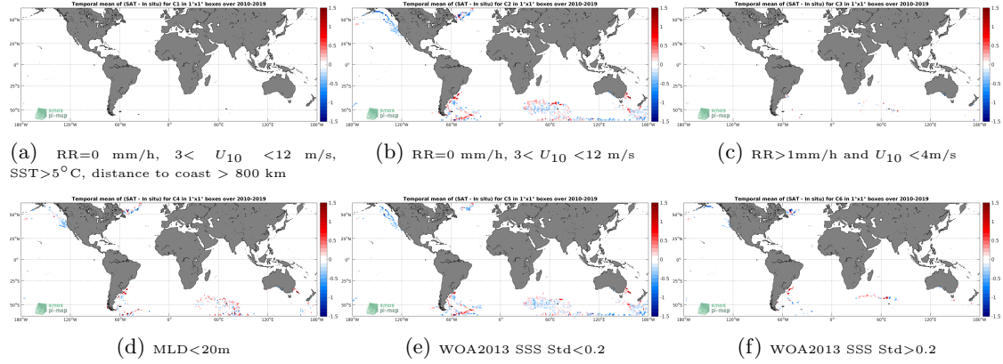
Figure 12: Temporal mean gridded over spatial boxes of size 1^{\circ} \times 1^{\circ} of \Delta\text{SSS} (SMOS SSS L3 v7 - 9 Days (CATDS-CECOS-LOCEAN) - Marine mammals) for 6 different subdatasets corresponding to: \text{RR}=0 mm/h, 3 < U_{10} < 12 m/s, \text{SST} > 5^{\circ}\text{C} , distance to coast > 800 km (a), \text{RR}=0 mm/h, 3 < U_{10} < 12 m/s (b), \text{RR} > 1\text{mm/h} and U_{10} < 4\text{m/s} (c), \text{MLD} < 20\text{m} (d), \text{WOA2013 SSS Std} < 0.2 (e), \text{WOA2013 SSS Std} > 0.2 (f).
