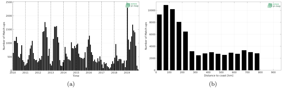
Figure 1: Number of match-ups between Marine mammals and SMOS SSS L3 v7 - 9 Days (CATDS-CECOS-LOCEAN) SSS as a function of time (a) and as function of the distance to coast (b) over the SMOS coastal zone (<800km) 60N-60S Pi-MEP region and for the full satellite product period.
