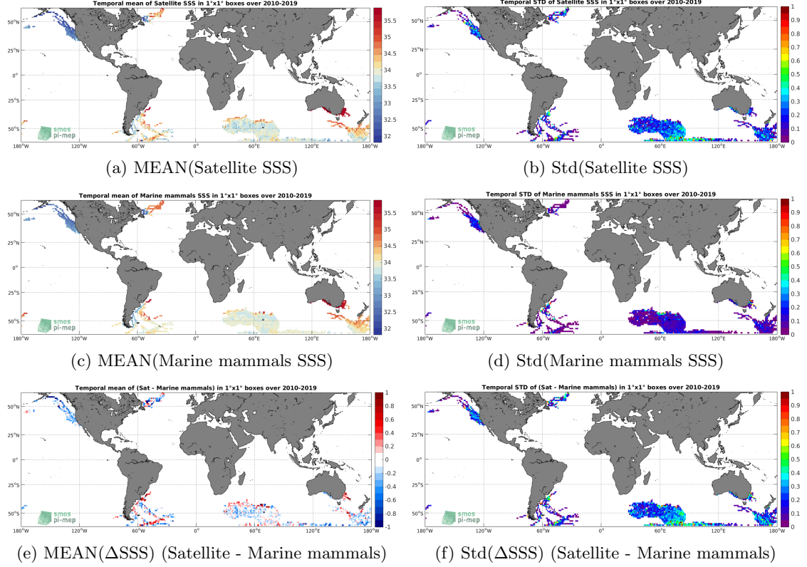
Figure 6: Temporal mean (left) and Std (right) of SSS from SMOS SSS L3 v7 - 9 Days (CATDS-CECOS-LOCEAN) (top), Marine mammals (middle), and of \Delta SSS (Satellite - Marine mammals). Only match-up pairs are used to generate these maps.
