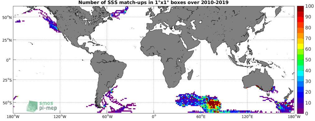
Figure 4: Number of SSS match-ups between Marine mammals SSS and the SMOS SSS L3 v7 - 9 Days (CATDS-CECOS-LOCEAN) SSS product for the SMOS coastal zone (<800km) 60N-60S Pi-MEP region over 1^\circ \times 1^\circ boxes and for the full satellite product period.
