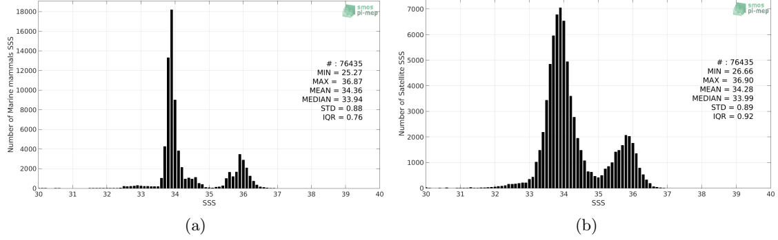
Figure 2: Histograms of SSS from Marine mammals (a) and SMOS SSS L3 v7 - 9 Days (CATDS-CECOS-LOCEAN) (b) considering all match-up pairs per bins of 0.1 over the SMOS coastal zone (<800km) 60N-60S Pi-MEP region and for the full satellite product period.
