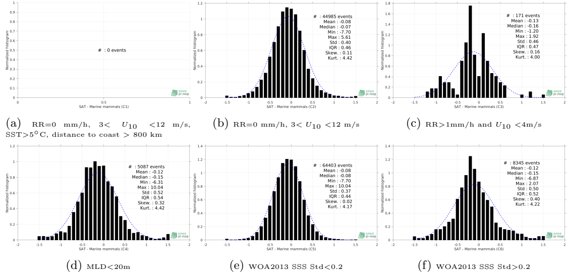
Figure 13: Normalized histogram of \Delta SSS (SMOS SSS L3 v7 - 9 Days (CATDS-CECOS-LOCEAN) - Marine mammals) for 6 different subdatasets corresponding to: RR=0 mm/h, 3 < U_{10} < 12 m/s, SST>5°C, distance to coast > 800 km (a), RR=0 mm/h, 3 < U_{10} < 12 m/s (b), RR>1mm/h and U_{10} < 4 m/s (c), MLD<20m (d), WOA2013 SSS Std<0.2 (e), WOA2013 SSS Std>0.2 (f).
