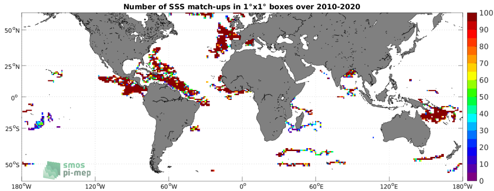
Figure 3: Number of SSS match-ups between Surface drifters SSS and the SMOS SSS L3 v7 - 9 Days (CATDS-CECOS-LOCEAN) SSS product for the SMOS coastal zone (<800km) 60N-60S Pi-MEP region over 1^\circ \times 1^\circ boxes and for the full satellite product period.
