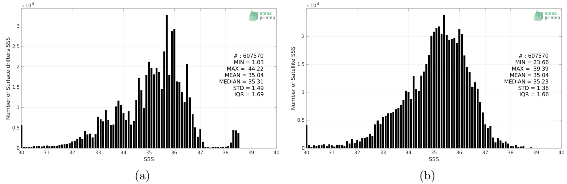
Figure 2: Histograms of SSS from Surface drifters (a) and SMOS SSS L3 v7 - 9 Days (CATDS-CECOS-LOCEAN) (b) considering all match-up pairs per bins of 0.1 over the SMOS coastal zone (<800km) 60N-60S Pi-MEP region and for the full satellite product period.
