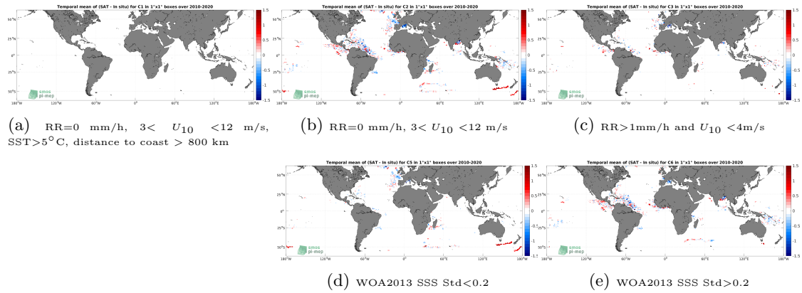
Figure 11: Temporal mean gridded over spatial boxes of size 1^\circ \times 1^\circ of \Delta\text{SSS} (SMOS SSS L3 v7 - 9 Days (CATDS-CECOS-LOCEAN) - Surface drifters) for 5 different subdatasets corresponding to:RR=0 mm/h, 3 < U_{10} < 12 m/s, SST >5^\circ\text{C} , distance to coast > 800 km (a), RR=0 mm/h, 3 < U_{10} < 12 m/s (b), RR >1 mm/h and U_{10} < 4 m/s (c), WOA2013 SSS Std <0.2 (d), WOA2013 SSS Std >0.2 (e).
