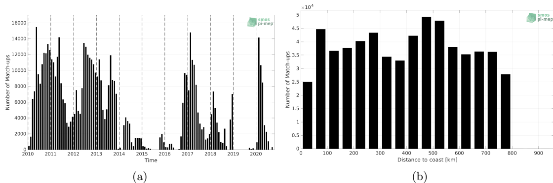
Figure 1: Number of match-ups between Surface drifters and SMOS SSS L3 v7 - 9 Days (CATDS-CECOS-LOCEAN) SSS as a function of time (a) and as function of the distance to coast (b) over the SMOS coastal zone (<800km) 60N-60S Pi-MEP region and for the full satellite product period.
