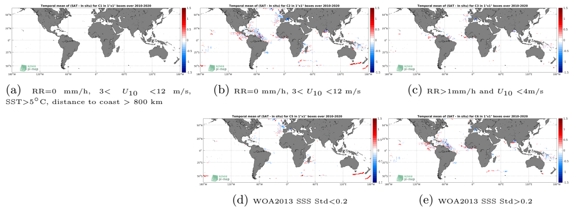
Figure 11: Temporal mean gridded over spatial boxes of size 1^\circ \times 1^\circ of \Delta SSS (SMOS SSS L3 v7 - 9 Days (CATDS-CECOS-LOCEAN) - Surface drifters) for 5 different subdatasets corresponding to:RR=0 mm/h, 3 < U_{10} < 12 m/s, SST >5^\circ C, distance to coast > 800 km (a), RR=0 mm/h, 3 < U_{10} < 12 m/s (b), RR >1 mm/h and U_{10} < 4 m/s (c), WOA2013 SSS Std <0.2 (d), WOA2013 SSS Std >0.2 (e).
