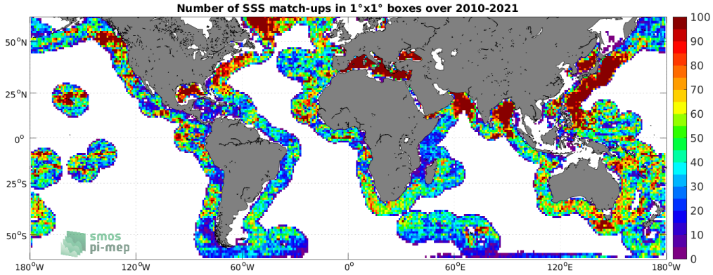
Figure 4: Number of SSS match-ups between Argo SSS and the SMOS SSS L3 v7 - 9 Days (CATDS-CECOS-LOCEAN) SSS product for the SMOS coastal zone (<800km) 60N-60S Pi-MEP region over 1^{\circ} \times 1^{\circ} boxes and for the full satellite product period.
