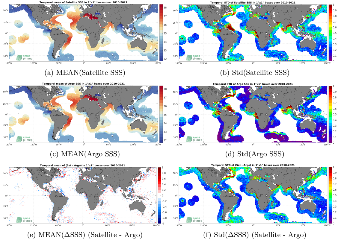
Figure 6: Temporal mean (left) and Std (right) of SSS from SMOS SSS L3 v7 - 9 Days (CATDS-CECOS-LOCEAN) (top), Argo (middle), and of \Delta SSS (Satellite - Argo). Only match-up pairs are used to generate these maps.
