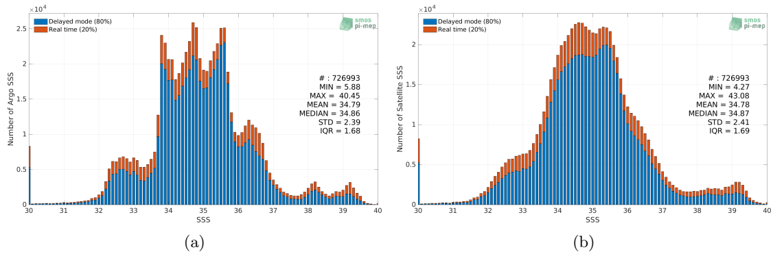
Figure 2: Histograms of SSS from Argo (a) and SMOS SSS L3 v7 - 9 Days (CATDS-CECOS-LOCEAN) (b) considering all match-up pairs per bins of 0.1 over the SMOS coastal zone (<800km) 60N-60S Pi-MEP region and for the full satellite product period.
