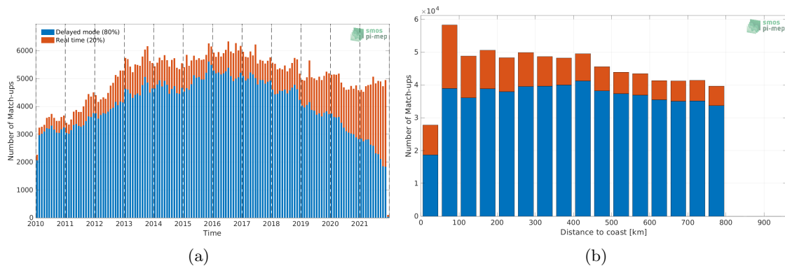
Figure 1: Number of match-ups between Argo and SMOS SSS L3 v7 - 9 Days (CATDS-CECOS-LOCEAN) SSS as a function of time (a) and as function of the distance to coast (b) over the SMOS coastal zone (<800km) 60N-60S Pi-MEP region and for the full satellite product period.
