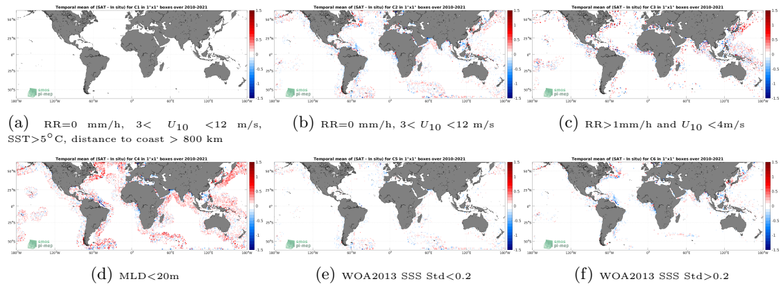
Figure 12: Temporal mean gridded over spatial boxes of size 1^\circ \times 1^\circ of \Delta SSS (SMOS SSS L3 v7 - 9 Days (CATDS-CECOS-LOCEAN) - Argo) for 6 different subdatasets corresponding to:RR=0 mm/h, 3 < U_{10} < 12 m/s, SST >5^\circ C, distance to coast > 800 km (a), RR=0 mm/h, 3 < U_{10} < 12 m/s (b), RR >1 mm/h and U_{10} < 4 m/s (c),MLD <20 m (d),WOA2013 SSS Std <0.2 (e),WOA2013 SSS Std >0.2 (f).
