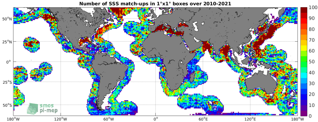
Figure 4: Number of SSS match-ups between Argo SSS and the SMOS SSS L3 v7 - 9 Days (CATDS-CECOS-LOCEAN) SSS product for the SMOS coastal zone (<800km) 60N-60S Pi-MEP region over 1^\circ \times 1^\circ boxes and for the full satellite product period.
