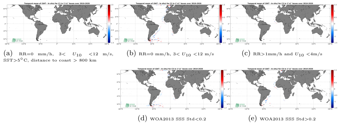
Figure 12: Temporal mean gridded over spatial boxes of size 1^\circ \times 1^\circ of \Delta SSS (SMOS SSS L3 v7 - 18 Days (CATDS-CECOS-LOCEAN) - TSG (Polarstern)) for 5 different subdatasets corresponding to:RR=0 mm/h, 3 < U_{10} < 12 m/s, SST > 5^\circ\text{C} , distance to coast > 800 km (a), RR=0 mm/h, 3 < U_{10} < 12 m/s (b), RR > 1 mm/h and U_{10} < 4 m/s (c), WOA2013 SSS Std < 0.2 (d), WOA2013 SSS Std > 0.2 (e).
