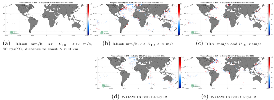
Figure 12: Temporal mean gridded over spatial boxes of size 1^\circ \times 1^\circ of \Delta SSS (SMOS SSS L3 v7 - 18 Days (CATDS-CECOS-LOCEAN) - TSG (LEGOS-DM)) for 5 different subdatasets corresponding to:RR=0 mm/h, 3 < U_{10} < 12 m/s, SST >5^\circ C, distance to coast > 800 km (a), RR=0 mm/h, 3 < U_{10} < 12 m/s (b), RR >1 mm/h and U_{10} < 4 m/s (c), WOA2013 SSS Std <0.2 (d), WOA2013 SSS Std >0.2 (e).
