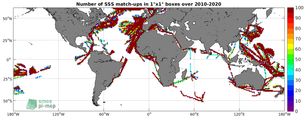
Figure 4: Number of SSS match-ups between TSG (LEGOS-DM) SSS and the SMOS SSS L3 v7 - 18 Days (CATDS-CECOS-LOCEAN) SSS product for the SMOS coastal zone ( <800\text{km} ) 60N-60S Pi-MEP region over 1^\circ \times 1^\circ boxes and for the full satellite product period.
