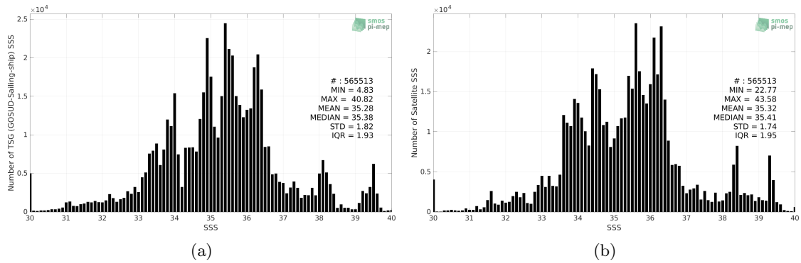
Figure 2: Histograms of SSS from TSG (GOSUD-Sailing-ship) (a) and SMOS SSS L3 v7 - 18 Days (CATDS-CECOS-LOCEAN) (b) considering all match-up pairs per bins of 0.1 over the SMOS coastal zone (<800km) 60N-60S Pi-MEP region and for the full satellite product period.
