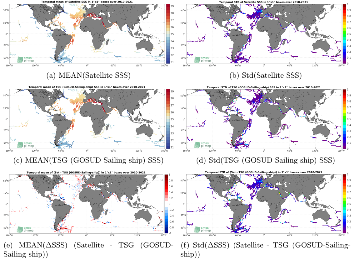
Figure 6: Temporal mean (left) and Std (right) of SSS from SMOS SSS L3 v7 - 18 Days (CATDS-CECOS-LOCEAN) (top), TSG (GOSUD-Sailing-ship) (middle), and of \Delta SSS (Satellite - TSG (GOSUD-Sailing-ship)). Only match-up pairs are used to generate these maps.
