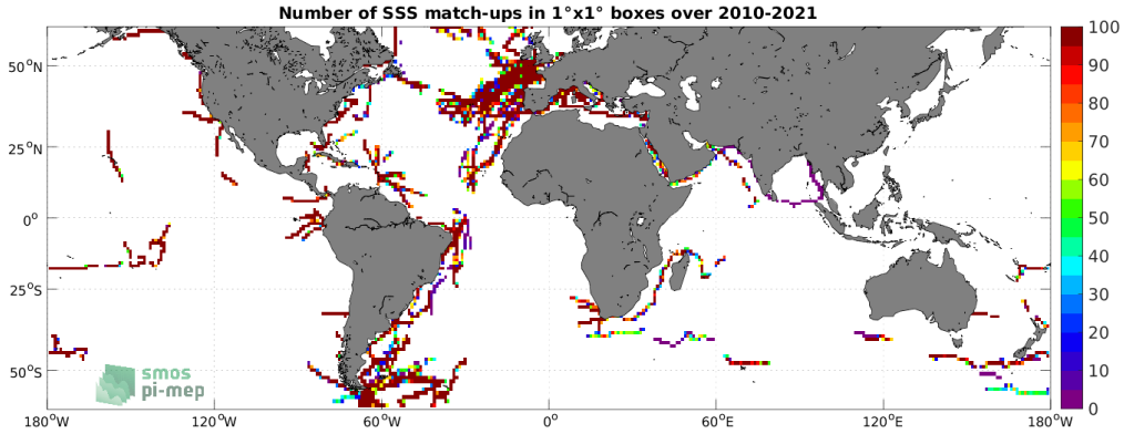
Figure 4: Number of SSS match-ups between TSG (GOSUD-Sailing-ship) SSS and the SMOS SSS L3 v7 - 18 Days (CATDS-CECOS-LOCEAN) SSS product for the SMOS coastal zone (<800km) 60N-60S Pi-MEP region over 1^\circ \times 1^\circ boxes and for the full satellite product period.
