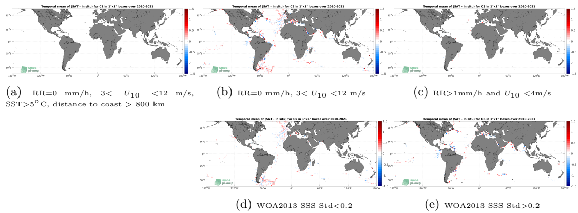
Figure 12: Temporal mean gridded over spatial boxes of size 1^\circ \times 1^\circ of \Delta\text{SSS} (SMOS SSS L3 v7 - 18 Days (CATDS-CECOS-LOCEAN) - TSG (GOSUD-Sailing-ship)) for 5 different subdatasets corresponding to:RR=0 mm/h, 3 < U_{10} < 12 m/s, SST >5^\circ\text{C} , distance to coast > 800 km (a), RR=0 mm/h, 3 < U_{10} < 12 m/s (b), RR >1 mm/h and U_{10} < 4 m/s (c), WOA2013 SSS Std <0.2 (d), WOA2013 SSS Std >0.2 (e).
