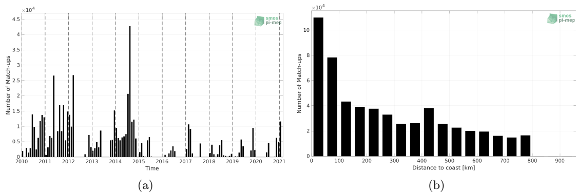
Figure 1: Number of match-ups between TSG (GOSUD-Sailing-ship) and SMOS SSS L3 v7 - 18 Days (CATDS-CECOS-LOCEAN) SSS as a function of time (a) and as function of the distance to coast (b) over the SMOS coastal zone (<800km) 60N-60S Pi-MEP region and for the full satellite product period.
