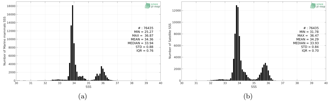
Figure 2: Histograms of SSS from Marine mammals (a) and SMOS SSS L3 v7 - 18 Days (CATDS-CECOS-LOCEAN) (b) considering all match-up pairs per bins of 0.1 over the SMOS coastal zone (<800km) 60N-60S Pi-MEP region and for the full satellite product period.
