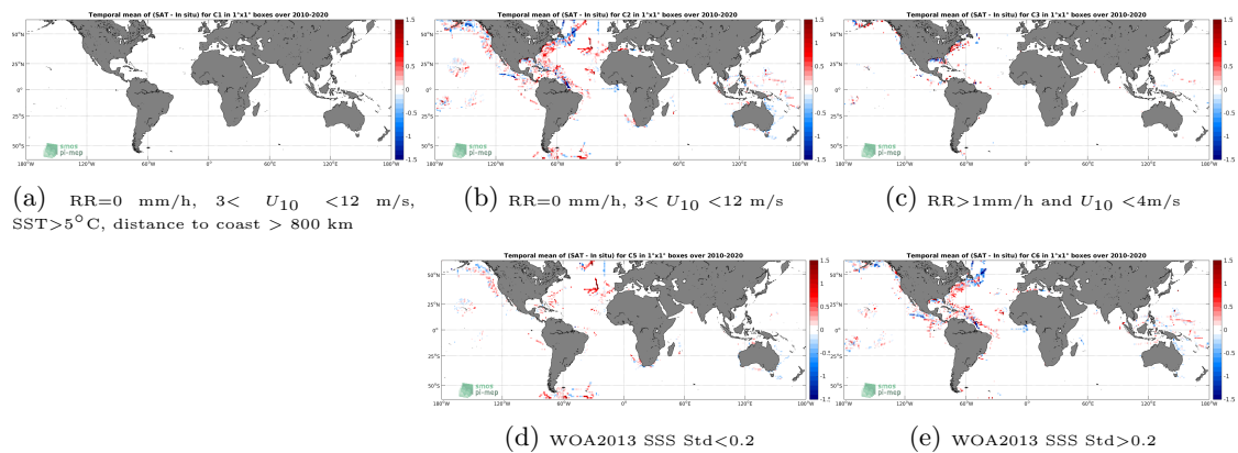
Figure 12: Temporal mean gridded over spatial boxes of size 1^\circ \times 1^\circ of \Delta\text{SSS} (SMOS SSS L3 v5 - 9 Days (CATDS-CECOS-LOCEAN) - TSG (SAMOS)) for 5 different subdatasets corresponding to:RR=0 mm/h, 3 < U_{10} < 12 m/s, SST >5^\circ\text{C} , distance to coast > 800 km (a), RR=0 mm/h, 3 < U_{10} < 12 m/s (b), RR >1 mm/h and U_{10} < 4 m/s (c), WOA2013 SSS Std <0.2 (d), WOA2013 SSS Std >0.2 (e).
