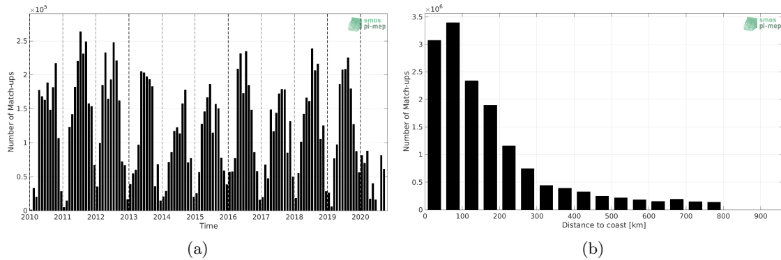
Figure 1: Number of match-ups between TSG (SAMOS) and SMOS SSS L3 v5 - 9 Days (CATDS-CECOS-LOCEAN) SSS as a function of time (a) and as function of the distance to coast (b) over the SMOS coastal zone (<800km) 60N-60S Pi-MEP region and for the full satellite product period.
