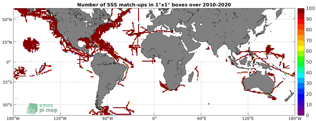
Figure 4: Number of SSS match-ups between TSG (SAMOS) SSS and the SMOS SSS L3 v5 - 9 Days (CATDS-CECOS-LOCEAN) SSS product for the SMOS coastal zone (<800km) 60N-60S Pi-MEP region over 1^\circ \times 1^\circ boxes and for the full satellite product period.
