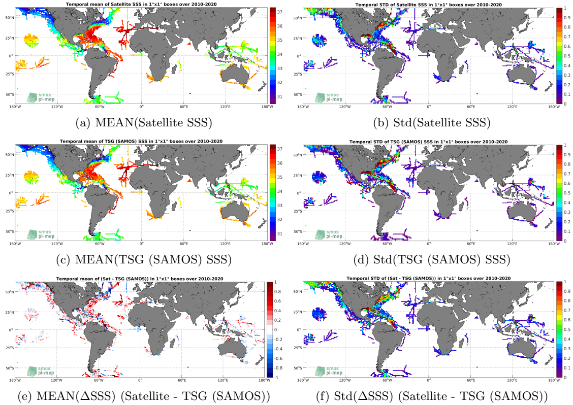
Figure 6: Temporal mean (left) and Std (right) of SSS from SMOS SSS L3 v5 - 9 Days (CATDS-CECOS-LOCEAN) (top), TSG (SAMOS) (middle), and of \Delta SSS (Satellite - TSG (SAMOS)). Only match-up pairs are used to generate these maps.
