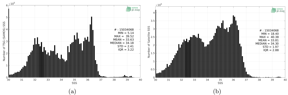
Figure 2: Histograms of SSS from TSG (SAMOS) (a) and SMOS SSS L3 v5 - 9 Days (CATDS-CECOS-LOCEAN) (b) considering all match-up pairs per bins of 0.1 over the SMOS coastal zone (<800km) 60N-60S Pi-MEP region and for the full satellite product period.
