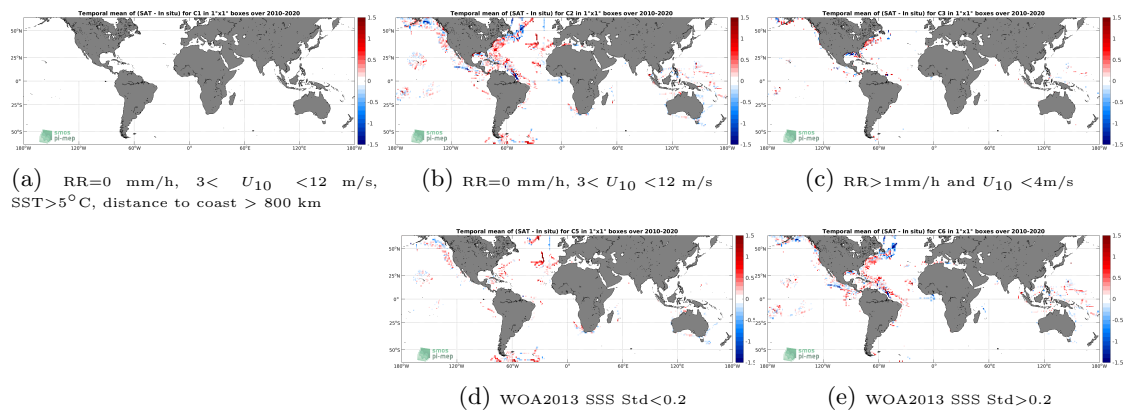
Figure 12: Temporal mean gridded over spatial boxes of size 1^\circ \times 1^\circ of \Delta SSS (SMOS SSS L3 v5 - 9 Days (CATDS-CECOS-LOCEAN) - TSG (SAMOS)) for 5 different subdatasets corresponding to:RR=0 mm/h, 3 < U_{10} < 12 m/s, SST >5^\circ C, distance to coast > 800 km (a), RR=0 mm/h, 3 < U_{10} < 12 m/s (b), RR >1 mm/h and U_{10} < 4 m/s (c), WOA2013 SSS Std <0.2 (d), WOA2013 SSS Std >0.2 (e).
