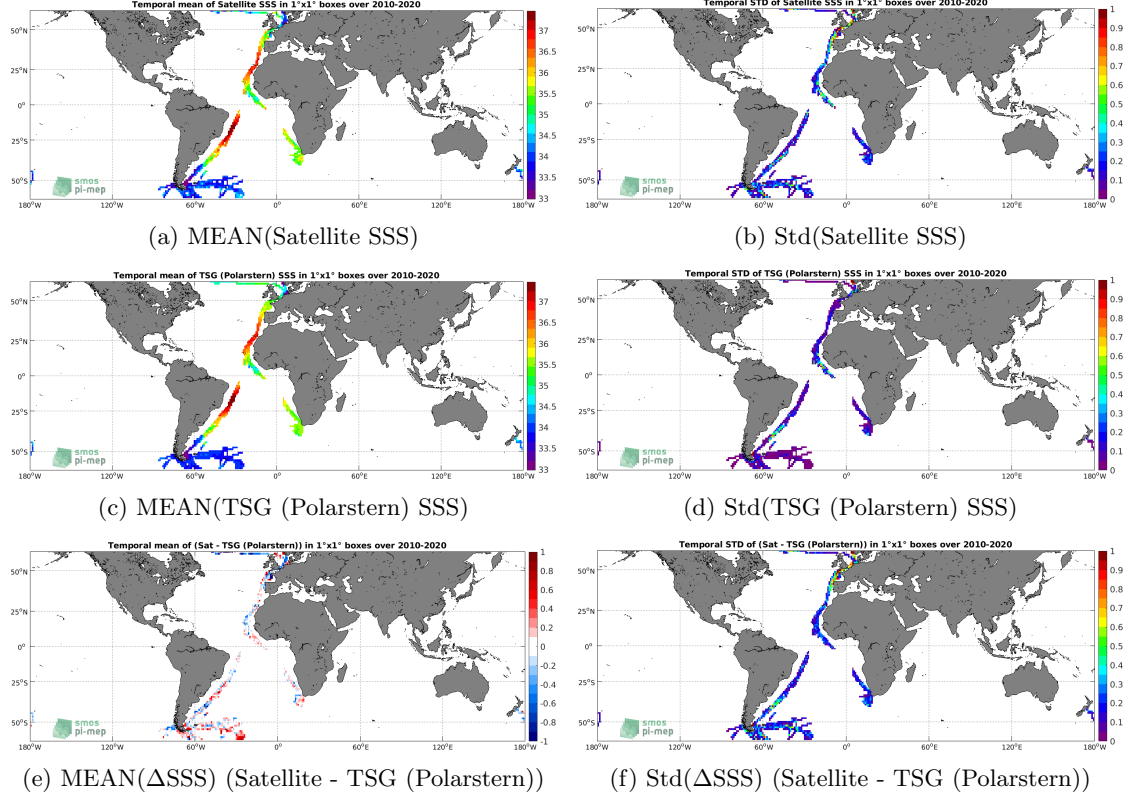
Figure 6: Temporal mean (left) and Std (right) of SSS from SMOS SSS L3 v5 - 9 Days (CATDS-CECOS-LOCEAN) (top), TSG (Polarstern) (middle), and of \Delta SSS (Satellite - TSG (Polarstern)). Only match-up pairs are used to generate these maps.
