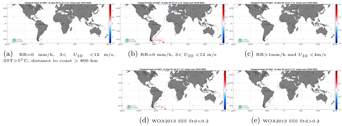
Figure 12: Temporal mean gridded over spatial boxes of size 1^\circ \times 1^\circ of \Delta SSS (SMOS SSS L3 v5 - 9 Days (CATDS-CECOS-LOCEAN) - TSG (Polarstern)) for 5 different subdatasets corresponding to: RR=0 mm/h, 3 < U_{10} < 12 m/s, SST > 5^\circ C , distance to coast > 800 km (a), RR=0 mm/h, 3 < U_{10} < 12 m/s (b), RR > 1 mm/h and U_{10} < 4 m/s (c), WOA2013 SSS Std < 0.2 (d), WOA2013 SSS Std > 0.2 (e).
