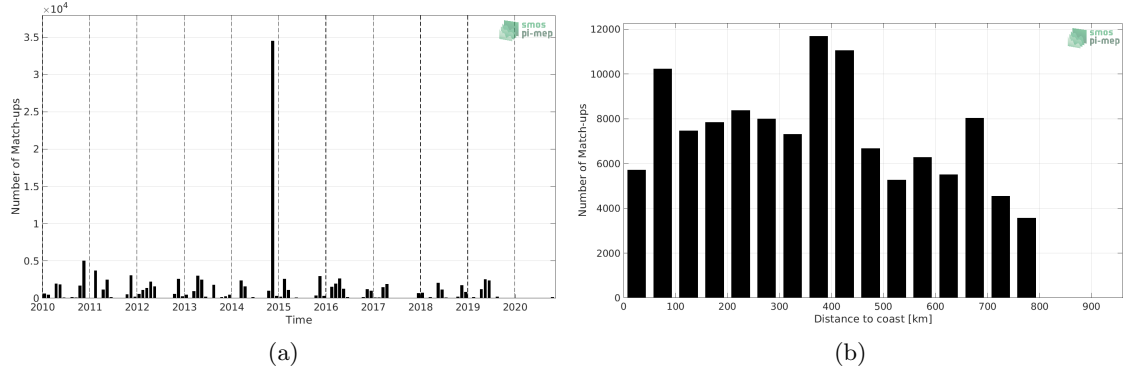
Figure 1: Number of match-ups between TSG (Polarstern) and SMOS SSS L3 v5 - 9 Days (CATDS-CECOS-LOCEAN) SSS as a function of time (a) and as function of the distance to coast (b) over the SMOS coastal zone (<800km) 60N-60S Pi-MEP region and for the full satellite product period.
