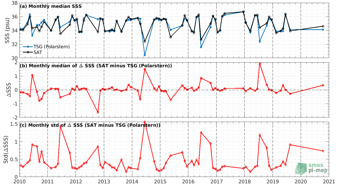
Figure 7: Time series of the monthly median SSS (top), median of \Delta SSS (Satellite - TSG (Polarstern)) and Std of \Delta SSS (Satellite - TSG (Polarstern)) over the SMOS coastal zone ( <800\text{km} ) 60N-60S Pi-MEP region considering all match-ups collected by the Pi-MEP.
