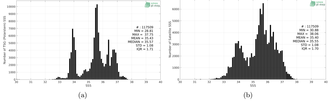
Figure 2: Histograms of SSS from TSG (Polarstern) (a) and SMOS SSS L3 v5 - 9 Days (CATDS-CECOS-LOCEAN) (b) considering all match-up pairs per bins of 0.1 over the SMOS coastal zone (<800km) 60N-60S Pi-MEP region and for the full satellite product period.
