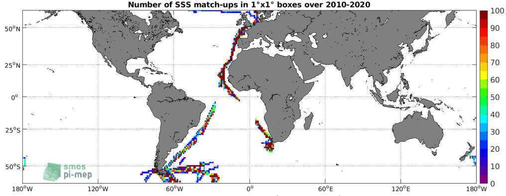
Figure 4: Number of SSS match-ups between TSG (Polarstern) SSS and the SMOS SSS L3 v5 - 9 Days (CATDS-CECOS-LOCEAN) SSS product for the SMOS coastal zone (<800km) 60N-60S Pi-MEP region over 1^\circ \times 1^\circ boxes and for the full satellite product period.
