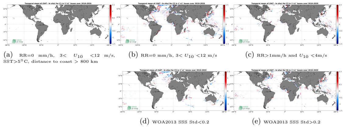
Figure 12: Temporal mean gridded over spatial boxes of size 1^\circ \times 1^\circ of \Delta SSS (SMOS SSS L3 v5 - 9 Days (CATDS-CECOS-LOCEAN) - TSG (LEGOS-DM)) for 5 different subdatasets corresponding to:RR=0 mm/h, 3 < U_{10} < 12 m/s, SST >5^\circ C, distance to coast > 800 km (a), RR=0 mm/h, 3 < U_{10} < 12 m/s (b), RR >1 mm/h and U_{10} < 4 m/s (c), WOA2013 SSS Std <0.2 (d), WOA2013 SSS Std >0.2 (e).
