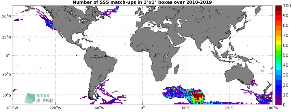
Figure 4: Number of SSS match-ups between Marine mammals SSS and the SMOS SSS L3 v5 - 9 Days (CATDS-CECOS-LOCEAN) SSS product for the SMOS coastal zone (<800km) 60N-60S Pi-MEP region over 1^\circ \times 1^\circ boxes and for the full satellite product period.
