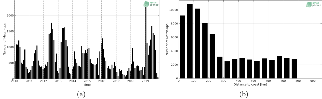
Figure 1: Number of match-ups between Marine mammals and SMOS SSS L3 v5 - 9 Days (CATDS-CECOS-LOCEAN) SSS as a function of time (a) and as function of the distance to coast (b) over the SMOS coastal zone (<800km) 60N-60S Pi-MEP region and for the full satellite product period.
