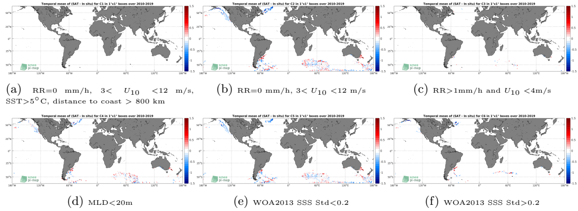
Figure 12: Temporal mean gridded over spatial boxes of size 1^{\circ} \times 1^{\circ} of \Delta\text{SSS} (SMOS SSS L3 v5 - 9 Days (CATDS-CECOS-LOCEAN) - Marine mammals) for 6 different subdatasets corresponding to: \text{RR}=0 \text{ mm/h} , 3 < U_{10} < 12 \text{ m/s} , \text{SST} > 5^{\circ}\text{C} , distance to coast > 800 \text{ km} (a), \text{RR}=0 \text{ mm/h} , 3 < U_{10} < 12 \text{ m/s} (b), \text{RR} > 1\text{mm/h} and U_{10} < 4\text{m/s} (c), \text{MLD} < 20\text{m} (d), \text{WOA2013 SSS Std} < 0.2 (e), \text{WOA2013 SSS Std} > 0.2 (f).
