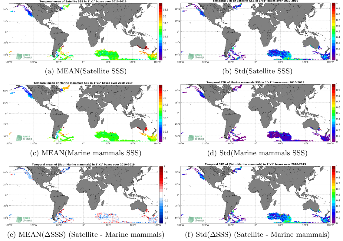
Figure 6: Temporal mean (left) and Std (right) of SSS from SMOS SSS L3 v5 - 9 Days (CATDS-CECOS-LOCEAN) (top), Marine mammals (middle), and of \Delta SSS (Satellite - Marine mammals). Only match-up pairs are used to generate these maps.
