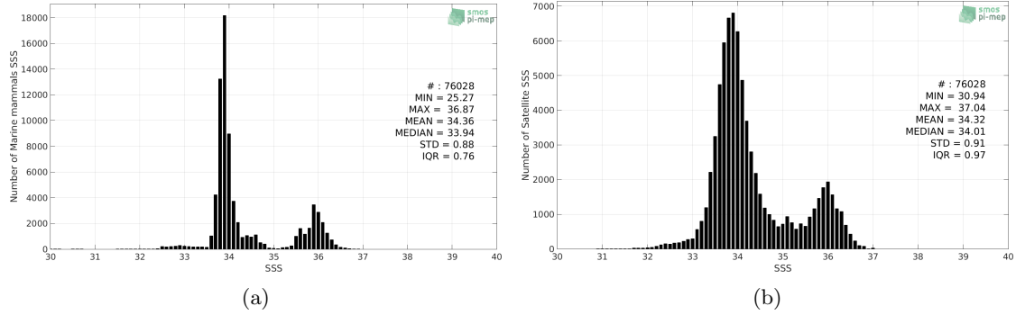
Figure 2: Histograms of SSS from Marine mammals (a) and SMOS SSS L3 v5 - 9 Days (CATDS-CECOS-LOCEAN) (b) considering all match-up pairs per bins of 0.1 over the SMOS coastal zone (<800km) 60N-60S Pi-MEP region and for the full satellite product period.
