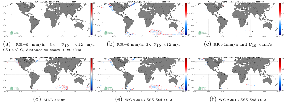
Figure 12: Temporal mean gridded over spatial boxes of size 1^\circ \times 1^\circ of \Delta SSS (SMOS SSS L3 v5 - 9 Days (CATDS-CECOS-LOCEAN) - Sea mammals) for 6 different subdatasets corresponding to: RR=0 mm/h, 3 < U_{10} < 12 m/s, SST > 5^\circ C , distance to coast > 800 km (a), RR=0 mm/h, 3 < U_{10} < 12 m/s (b), RR > 1 mm/h and U_{10} < 4 m/s (c), MLD < 20 m (d), WOA2013 SSS Std < 0.2 (e), WOA2013 SSS Std > 0.2 (f).
