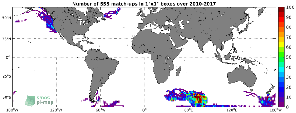
Figure 4: Number of SSS match-ups between Sea mammals SSS and the SMOS SSS L3 v5 - 9 Days (CATDS-CECOS-LOCEAN) SSS product for the SMOS coastal zone (<800km) 60N-60S Pi-MEP region over 1°x1° boxes and for the full satellite product period.
