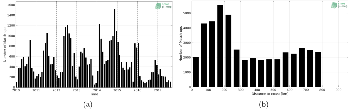
Figure 1: Number of match-ups between Sea mammals and SMOS SSS L3 v5 - 9 Days (CATDS-CECOS-LOCEAN) SSS as a function of time (a) and as function of the distance to coast (b) over the SMOS coastal zone (<800km) 60N-60S Pi-MEP region and for the full satellite product period.
