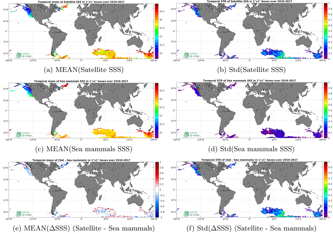
Figure 6: Temporal mean (left) and Std (right) of SSS from SMOS SSS L3 v5 - 9 Days (CATDS-CECOS-LOCEAN) (top), Sea mammals (middle), and of \Delta SSS (Satellite - Sea mammals). Only match-up pairs are used to generate these maps.
