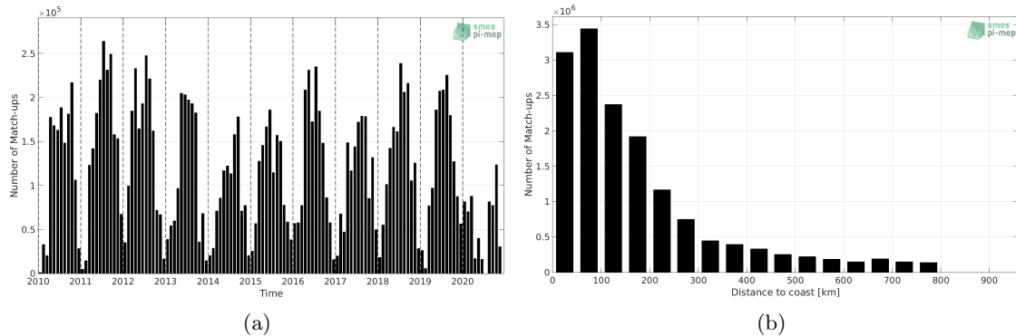
Figure 1: Number of match-ups between TSG (SAMOS) and SMOS SSS L3 v5 - 18 Days (CATDS-CECOS-LOCEAN) SSS as a function of time (a) and as function of the distance to coast (b) over the SMOS coastal zone (<800km) 60N-60S Pi-MEP region and for the full satellite product period.
