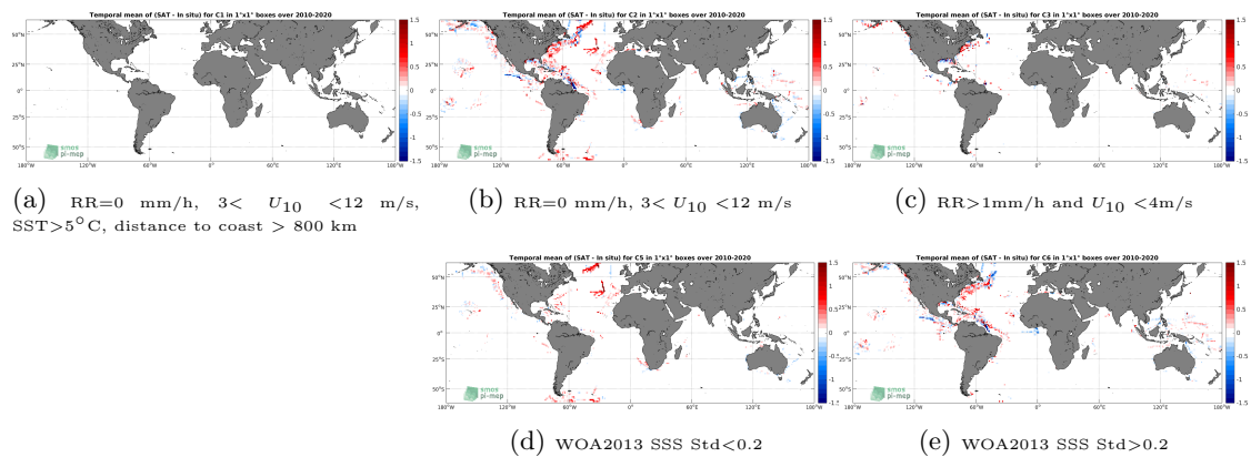
Figure 12: Temporal mean gridded over spatial boxes of size 1^\circ \times 1^\circ of \Delta\text{SSS} (SMOS SSS L3 v5 - 18 Days (CATDS-CECOS-LOCEAN) - TSG (SAMOS)) for 5 different subdatasets corresponding to:RR=0 mm/h, 3 < U_{10} < 12 m/s, SST>5°C, distance to coast > 800 km (a), RR=0 mm/h, 3 < U_{10} < 12 m/s (b), RR>1mm/h and U_{10} < 4 m/s (c), WOA2013 SSS Std<0.2 (d), WOA2013 SSS Std>0.2 (e).
