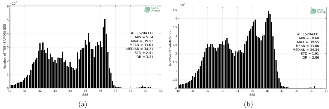
Figure 2: Histograms of SSS from TSG (SAMOS) (a) and SMOS SSS L3 v5 - 18 Days (CATDS-CECOS-LOCEAN) (b) considering all match-up pairs per bins of 0.1 over the SMOS coastal zone (<800km) 60N-60S Pi-MEP region and for the full satellite product period.
