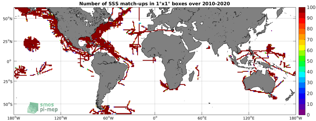
Figure 4: Number of SSS match-ups between TSG (SAMOS) SSS and the SMOS SSS L3 v5 - 18 Days (CATDS-CECOS-LOCEAN) SSS product for the SMOS coastal zone (<800km) 60N-60S Pi-MEP region over 1^{\circ} \times 1^{\circ} boxes and for the full satellite product period.
