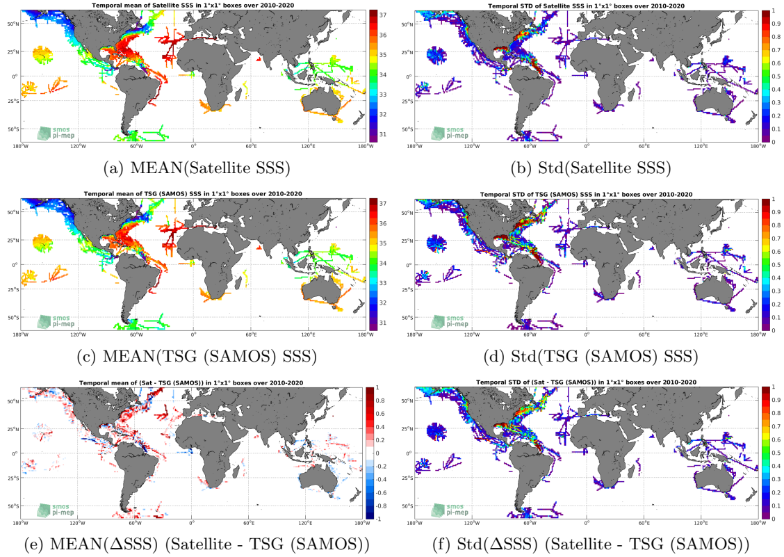
Figure 6: Temporal mean (left) and Std (right) of SSS from SMOS SSS L3 v5 - 18 Days (CATDS-CECOS-LOCEAN) (top), TSG (SAMOS) (middle), and of \Delta SSS (Satellite - TSG (SAMOS)). Only match-up pairs are used to generate these maps.
