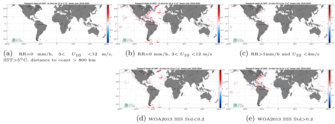
Figure 12: Temporal mean gridded over spatial boxes of size 1^\circ \times 1^\circ of \Delta SSS (SMOS SSS L3 v5 - 18 Days (CATDS-CECOS-LOCEAN) - TSG (SAMOS)) for 5 different subdatasets corresponding to: RR=0 mm/h, 3 < U_{10} < 12 m/s, SST > 5°C, distance to coast > 800 km (a), RR=0 mm/h, 3 < U_{10} < 12 m/s (b), RR > 1mm/h and U_{10} < 4 m/s (c), WOA2013 SSS Std < 0.2 (d), WOA2013 SSS Std > 0.2 (e).
