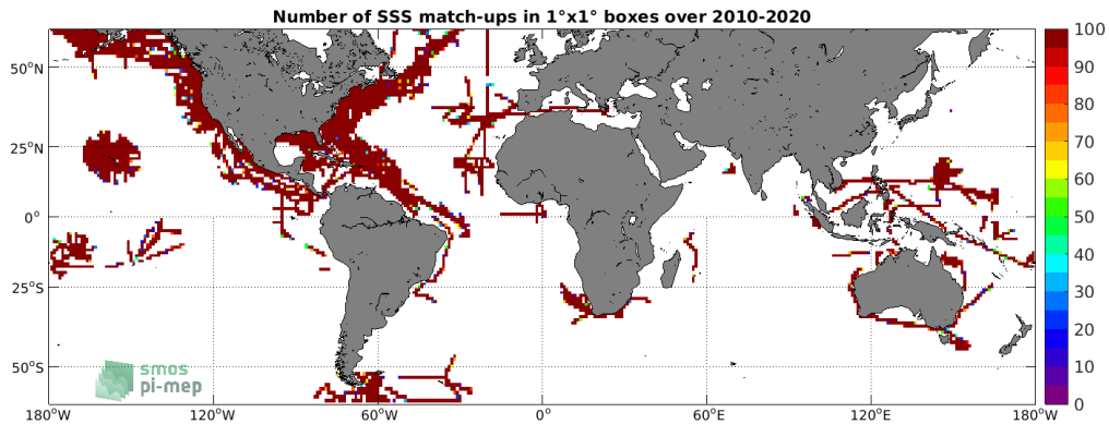
Figure 4: Number of SSS match-ups between TSG (SAMOS) SSS and the SMOS SSS L3 v5 - 18 Days (CATDS-CECOS-LOCEAN) SSS product for the SMOS coastal zone (<800km) 60N-60S Pi-MEP region over 1^\circ \times 1^\circ boxes and for the full satellite product period.
