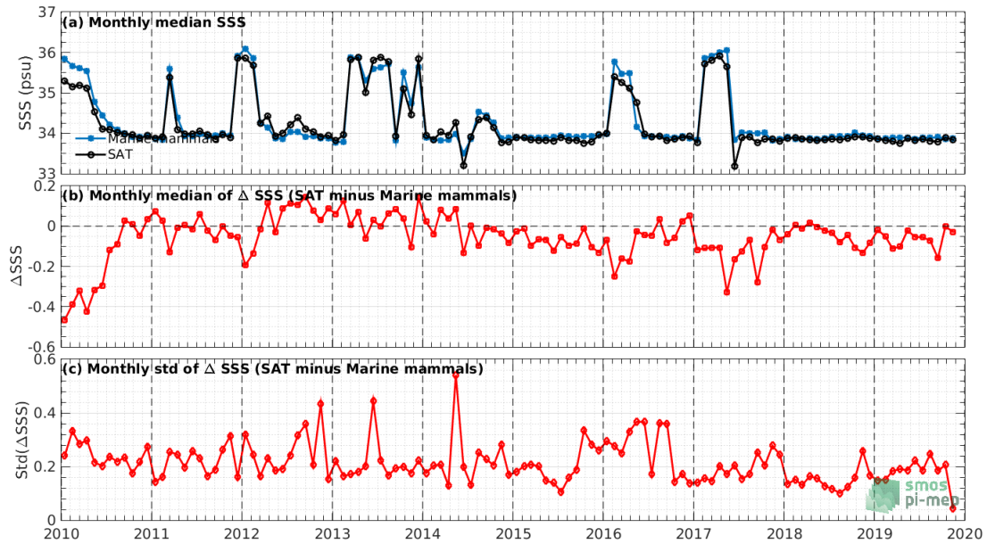
Figure 7: Time series of the monthly median SSS (top), median of \Delta SSS (Satellite - Marine mammals) over the SMOS coastal zone ( <800\text{km} ) 60N-60S Pi-MEP region considering all match-ups collected by the Pi-MEP.
