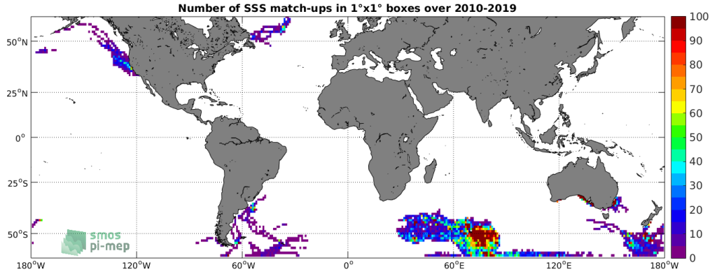
Figure 4: Number of SSS match-ups between Marine mammals SSS and the SMOS SSS L3 v5 - 18 Days (CATDS-CECOS-LOCEAN) SSS product for the SMOS coastal zone (<800km) 60N-60S Pi-MEP region over 1^\circ \times 1^\circ boxes and for the full satellite product period.
