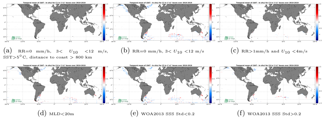
Figure 12: Temporal mean gridded over spatial boxes of size 1^{\circ}\times 1^{\circ} of \Delta\text{SSS} (SMOS SSS L3 v5 - 18 Days (CATDS-CECOS-LOCEAN) - Marine mammals) for 6 different subdatasets corresponding to:RR=0 mm/h, 3 < U_{10} < 12 m/s, SST >5^{\circ}\text{C} , distance to coast > 800 km (a), RR=0 mm/h, 3 < U_{10} < 12 m/s (b), RR >1\text{mm/h} and U_{10} < 4\text{m/s} (c),MLD <20\text{m} (d),WOA2013 SSS Std <0.2 (e),WOA2013 SSS Std >0.2 (f).
