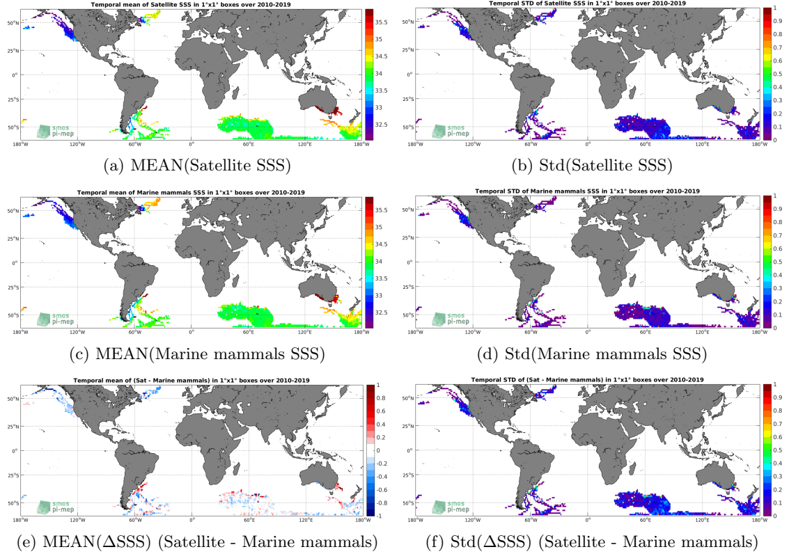
Figure 6: Temporal mean (left) and Std (right) of SSS from SMOS SSS L3 v5 - 18 Days (CATDS-CECOS-LOCEAN) (top), Marine mammals (middle), and of \Delta SSS (Satellite - Marine mammals). Only match-up pairs are used to generate these maps.
