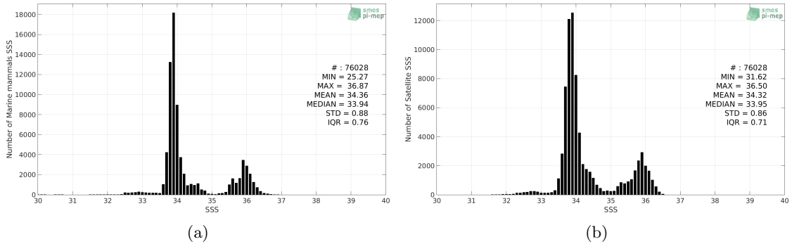
Figure 2: Histograms of SSS from Marine mammals (a) and SMOS SSS L3 v5 - 18 Days (CATDS-CECOS-LOCEAN) (b) considering all match-up pairs per bins of 0.1 over the SMOS coastal zone (<800km) 60N-60S Pi-MEP region and for the full satellite product period.
