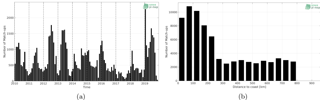
Figure 1: Number of match-ups between Marine mammals and SMOS SSS L3 v5 - 18 Days (CATDS-CECOS-LOCEAN) SSS as a function of time (a) and as function of the distance to coast (b) over the SMOS coastal zone (<800km) 60N-60S Pi-MEP region and for the full satellite product period.
