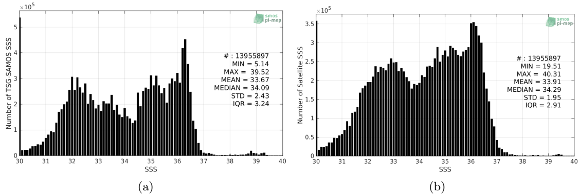
Figure 2: Histograms of SSS from TSG-SAMOS (a) and SMOS-L3-CATDS-CECOS-LOCEAN-V4-9DAYS-25KM (b) considering all match-up pairs per bins of 0.1 over the SMOS coastal zone ( \leq 800 km) 60N-60S Pi-MEP region and for the full satellite product period.
