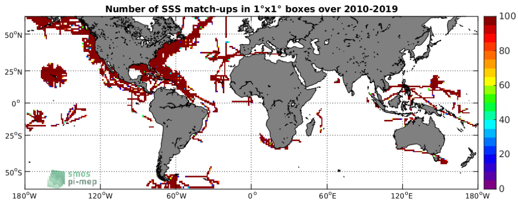
Figure 4: Number of SSS match-ups between TSG-SAMOS SSS and the SMOS-L3-CATDS-CECOS-LOCEAN-V4-9DAYS-25KM SSS product for the SMOS coastal zone ( \approx 800\text{km} ) 60N-60S Pi-MEP region over 1^\circ \times 1^\circ boxes and for the full satellite product period.
