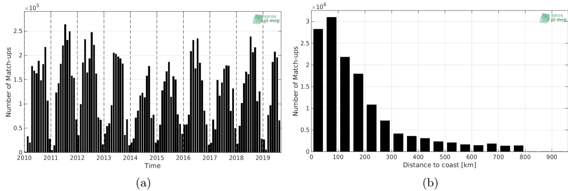
Figure 1: Number of match-ups between TSG-SAMOS and SMOS-L3-CATDS-CECOS-LOCEAN-V4-9DAYS-25KM SSS as a function of time (a) and as function of the distance to coast (b) over the SMOS coastal zone ( \leq 800 km) 60N-60S Pi-MEP region and for the full satellite product period.
