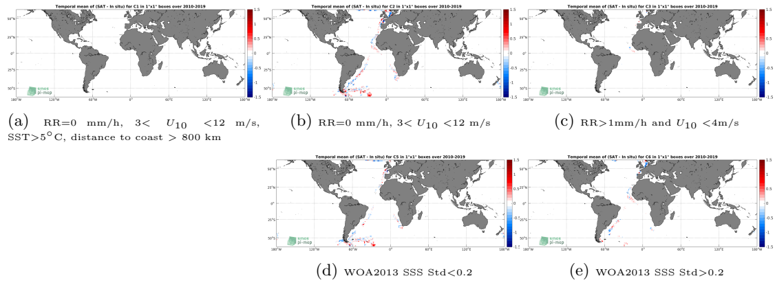
Figure 12: Temporal mean gridded over spatial boxes of size 1^\circ \times 1^\circ of \Delta SSS (SMOS SSS L3 v4 - 9 Days (CATDS-CECOS-LOCEAN) - TSG (Polarstern)) for 5 different subdatasets corresponding to: RR=0 mm/h, 3 < U_{10} < 12 m/s, SST > 5^\circ C , distance to coast > 800 km (a), RR=0 mm/h, 3 < U_{10} < 12 m/s (b), RR > 1 mm/h and U_{10} < 4 m/s (c), WOA2013 SSS Std < 0.2 (d), WOA2013 SSS Std > 0.2 (e).
