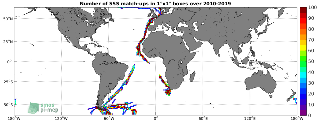
Figure 4: Number of SSS match-ups between TSG (Polarstern) SSS and the SMOS SSS L3 v4 - 9 Days (CATDS-CECOS-LOCEAN) SSS product for the SMOS coastal zone (<800km) 60N-60S Pi-MEP region over 1^\circ \times 1^\circ boxes and for the full satellite product period.
