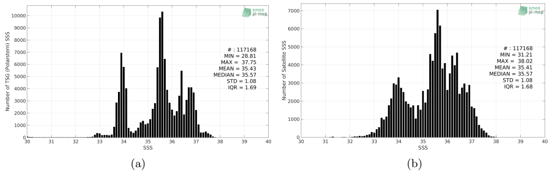
Figure 2: Histograms of SSS from TSG (Polarstern) (a) and SMOS SSS L3 v4 - 9 Days (CATDS-CECOS-LOCEAN) (b) considering all match-up pairs per bins of 0.1 over the SMOS coastal zone (<800km) 60N-60S Pi-MEP region and for the full satellite product period.
