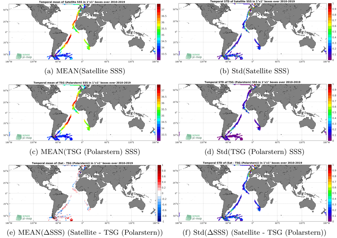
Figure 6: Temporal mean (left) and Std (right) of SSS from SMOS SSS L3 v4 - 9 Days (CATDS-CECOS-LOCEAN) (top), TSG (Polarstern) (middle), and of \Delta SSS (Satellite - TSG (Polarstern)). Only match-up pairs are used to generate these maps.
