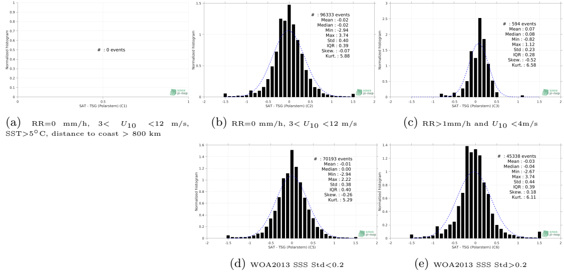
Figure 13: Normalized histogram of \Delta SSS (SMOS SSS L3 v4 - 9 Days (CATDS-CECOS-LOCEAN) - TSG (Polarstern)) for 5 different subdatasets corresponding to: RR=0 mm/h, 3 < U_{10} < 12 m/s, SST>5°C, distance to coast > 800 km (a), RR=0 mm/h, 3 < U_{10} < 12 m/s (b), RR>1mm/h and U_{10} < 4 m/s (c), WOA2013 SSS Std<0.2 (d), WOA2013 SSS Std>0.2 (e).
