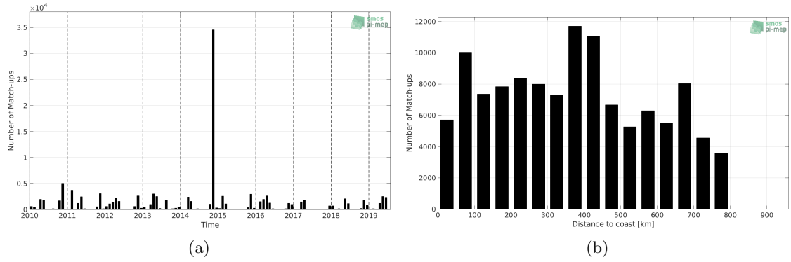
Figure 1: Number of match-ups between TSG (Polarstern) and SMOS SSS L3 v4 - 9 Days (CATDS-CECOS-LOCEAN) SSS as a function of time (a) and as function of the distance to coast (b) over the SMOS coastal zone (<800km) 60N-60S Pi-MEP region and for the full satellite product period.
