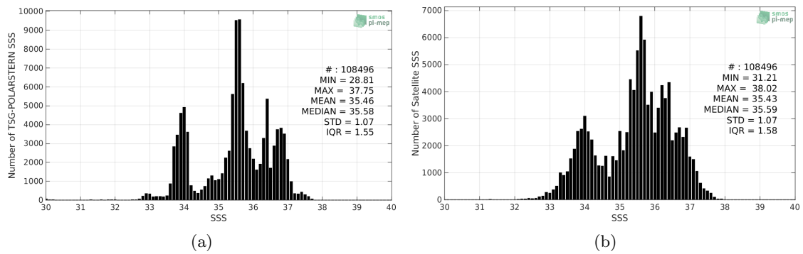
Figure 2: Histograms of SSS from TSG-POLARSTERN (a) and SMOS-L3-CATDS-CECOS-LOCEAN-V4-9DAYS-25KM (b) considering all match-up pairs per bins of 0.1 over the SMOS coastal zone ( \geq 800 km) 60N-60S Pi-MEP region and for the full satellite product period.
