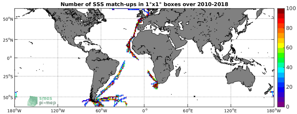
Figure 4: Number of SSS match-ups between TSG-POLARSTERN SSS and the SMOS-L3-CATDS-CECOS-LOCEAN-V4-9DAYS-25KM SSS product for the SMOS coastal zone ( \geq 800 km) 60N-60S Pi-MEP region over 1^\circ \times 1^\circ boxes and for the full satellite product period.
