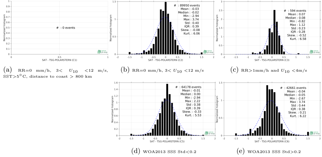
Figure 13: Normalized histogram of \Delta\text{SSS} (SMOS-L3-CATDS-CECOS-LOCEAN-V4-9DAYS-25KM - TSG-POLARSTERN) for 5 different sub-datasets corresponding to: RR=0 mm/h, 3 < U_{10} < 12 m/s, SST > 5^\circ\text{C} , distance to coast > 800 km (a), RR=0 mm/h, 3 < U_{10} < 12 m/s (b), RR > 1\text{mm/h} and U_{10} < 4\text{m/s} (c), WOA2013 SSS Std <0.2 (d), WOA2013 SSS Std >0.2 (e).
