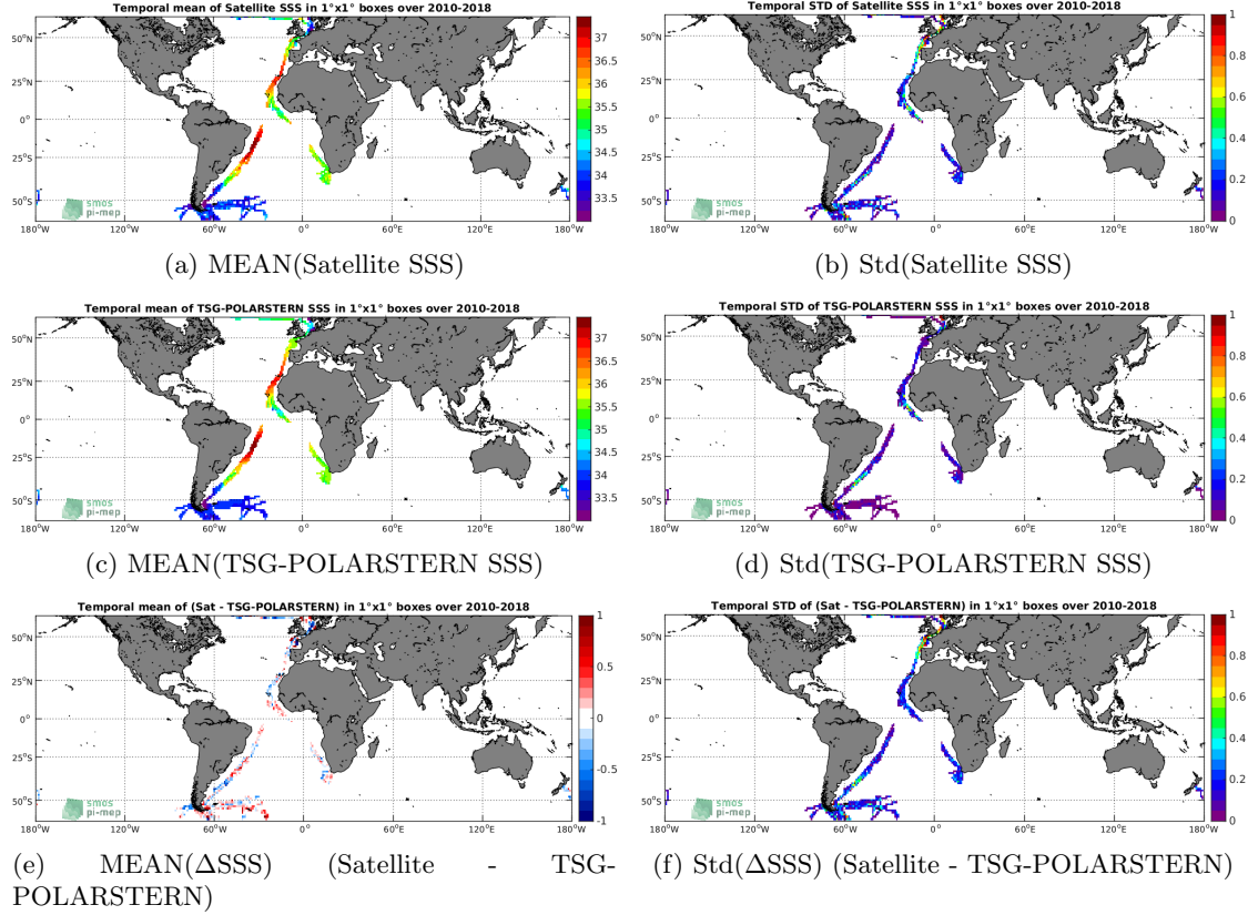
Figure 6: Temporal mean (left) and Std (right) of SSS from SMOS-L3-CATDS-CECOS-LOCEAN-V4-9DAYS-25KM (top), TSG-POLARSTERN (middle), and of \Delta SSS (Satellite - TSG-POLARSTERN). Only match-up pairs are used to generate these maps.
