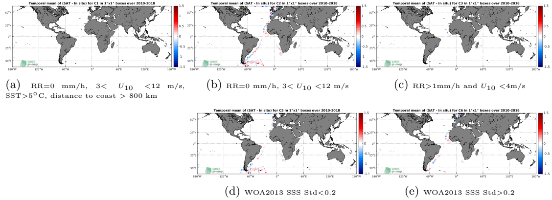
Figure 12: Temporal mean gridded over spatial boxes of size 1^\circ \times 1^\circ of \Delta SSS (SMOS-L3-CATDS-CECOS-LOCEAN-V4-9DAYS-25KM - TSG-POLARSTERN) for 5 different subdatasets corresponding to: RR=0 mm/h, 3 < U_{10} < 12 m/s, SST > 5^\circ C , distance to coast > 800 km (a), RR=0 mm/h, 3 < U_{10} < 12 m/s (b), RR > 1 mm/h and U_{10} < 4 m/s (c), WOA2013 SSS Std < 0.2 (d), WOA2013 SSS Std > 0.2 (e).
