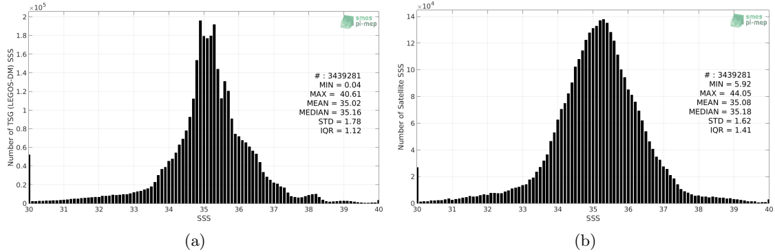
Figure 2: Histograms of SSS from TSG (LEGOS-DM) (a) and SMOS SSS L3 v4 - 9 Days (CATDS-CECOS-LOCEAN) (b) considering all match-up pairs per bins of 0.1 over the SMOS coastal zone (<800km) 60N-60S Pi-MEP region and for the full satellite product period.
