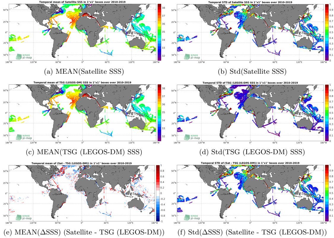
Figure 6: Temporal mean (left) and Std (right) of SSS from SMOS SSS L3 v4 - 9 Days (CATDS-CECOS-LOCEAN) (top), TSG (LEGOS-DM) (middle), and of \Delta SSS (Satellite - TSG (LEGOS-DM)). Only match-up pairs are used to generate these maps.
