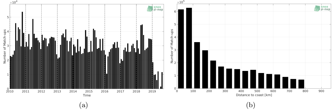
Figure 1: Number of match-ups between TSG (LEGOS-DM) and SMOS SSS L3 v4 - 9 Days (CATDS-CECOS-LOCEAN) SSS as a function of time (a) and as function of the distance to coast (b) over the SMOS coastal zone (<800km) 60N-60S Pi-MEP region and for the full satellite product period.
