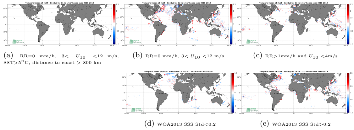
Figure 12: Temporal mean gridded over spatial boxes of size 1^\circ \times 1^\circ of \Delta SSS (SMOS SSS L3 v4 - 9 Days (CATDS-CECOS-LOCEAN) - TSG (LEGOS-DM)) for 5 different subdatasets corresponding to: RR=0 mm/h, 3 < U_{10} < 12 m/s, SST > 5^\circ C , distance to coast > 800 km (a), RR=0 mm/h, 3 < U_{10} < 12 m/s (b), RR > 1 mm/h and U_{10} < 4 m/s (c), WOA2013 SSS Std < 0.2 (d), WOA2013 SSS Std > 0.2 (e).
