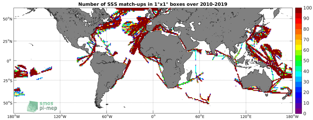
Figure 4: Number of SSS match-ups between TSG (LEGOS-DM) SSS and the SMOS SSS L3 v4 - 9 Days (CATDS-CECOS-LOCEAN) SSS product for the SMOS coastal zone (<800km) 60N-60S Pi-MEP region over 1°x1° boxes and for the full satellite product period.
