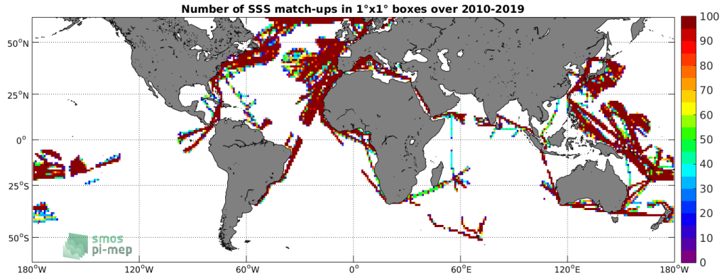
Figure 4: Number of SSS match-ups between TSG-LEGOS-DM SSS and the SMOS-L3-CATDS-CECOS-LOCEAN-V4-9DAYS-25KM SSS product for the SMOS coastal zone (<800km) 60N-60S Pi-MEP region over 1°x1° boxes and for the full satellite product period.
