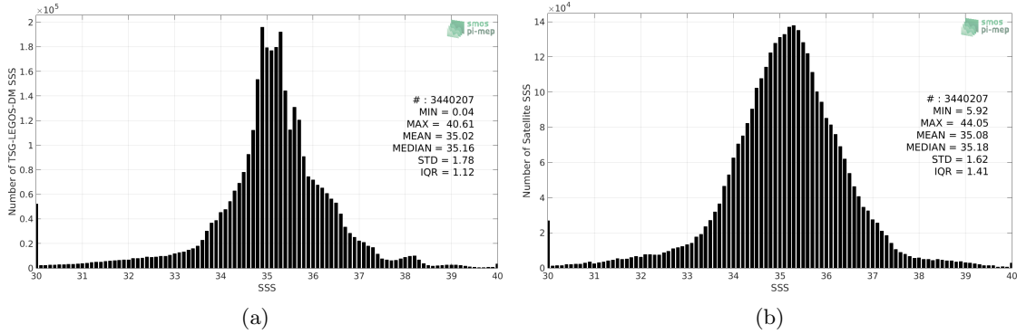
Figure 2: Histograms of SSS from TSG-LEGOS-DM (a) and SMOS-L3-CATDS-CECOS-LOCEAN-V4-9DAYS-25KM (b) considering all match-up pairs per bins of 0.1 over the SMOS coastal zone (<800km) 60N-60S Pi-MEP region and for the full satellite product period.
