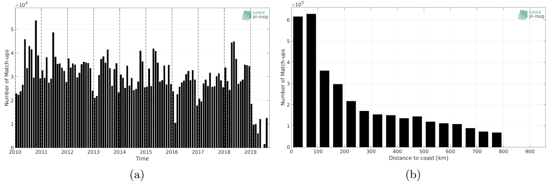
Figure 1: Number of match-ups between TSG-LEGOS-DM and SMOS-L3-CATDS-CECOS-LOCEAN-V4-9DAYS-25KM SSS as a function of time (a) and as function of the distance to coast (b) over the SMOS coastal zone (<800km) 60N-60S Pi-MEP region and for the full satellite product period.
