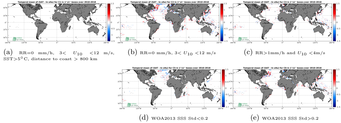
Figure 12: Temporal mean gridded over spatial boxes of size 1^\circ \times 1^\circ of \Delta SSS (SMOS-L3-CATDS-CECOS-LOCEAN-V4-9DAYS-25KM - TSG-LEGOS-DM) for 5 different subdatasets corresponding to: RR=0 mm/h, 3 < U_{10} < 12 m/s, SST > 5^\circ C , distance to coast > 800 km (a), RR=0 mm/h, 3 < U_{10} < 12 m/s (b), RR > 1 mm/h and U_{10} < 4 m/s (c), WOA2013 SSS Std < 0.2 (d), WOA2013 SSS Std > 0.2 (e).
