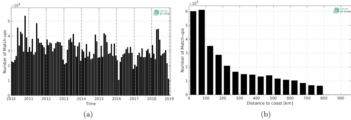
Figure 1: Number of match-ups between TSG-LEGOS-DM and SMOS-L3-CATDS-CECOS-LOCEAN-V4-9DAYS-25KM SSS as a function of time (a) and as function of the distance to coast (b) over the SMOS coastal zone ( \leq 800 km) 60N-60S Pi-MEP region and for the full satellite product period.
