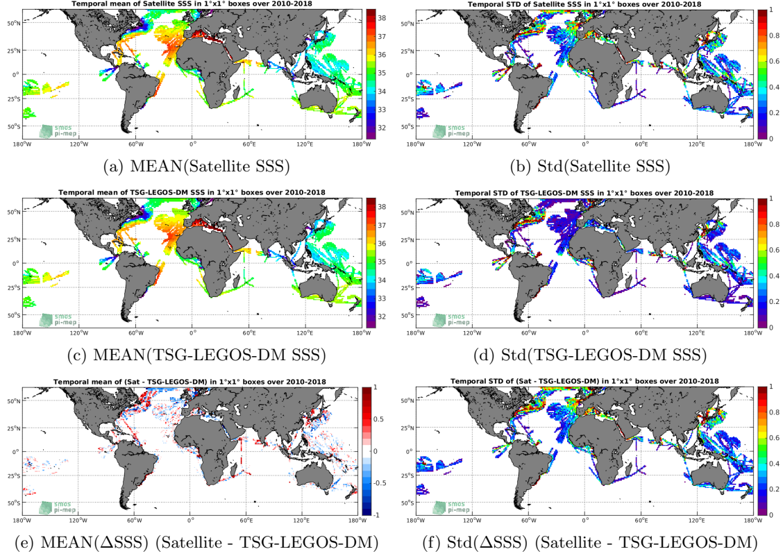
Figure 6: Temporal mean (left) and Std (right) of SSS from SMOS-L3-CATDS-CECOS-LOCEAN-V4-9DAYS-25KM (top), TSG-LEGOS-DM (middle), and of \Delta SSS (Satellite - TSG-LEGOS-DM). Only match-up pairs are used to generate these maps.
