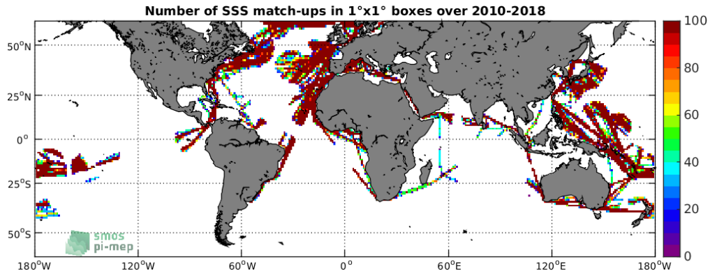
Figure 4: Number of SSS match-ups between TSG-LEGOS-DM SSS and the SMOS-L3-CATDS-CECOS-LOCEAN-V4-9DAYS-25KM SSS product for the SMOS coastal zone ( \leq 800\text{km} ) 60N-60S Pi-MEP region over 1^\circ \times 1^\circ boxes and for the full satellite product period.
