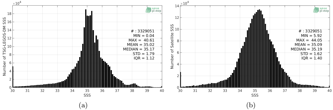
Figure 2: Histograms of SSS from TSG-LEGOS-DM (a) and SMOS-L3-CATDS-CECOS-LOCEAN-V4-9DAYS-25KM (b) considering all match-up pairs per bins of 0.1 over the SMOS coastal zone ( \leq 800 km) 60N-60S Pi-MEP region and for the full satellite product period.
