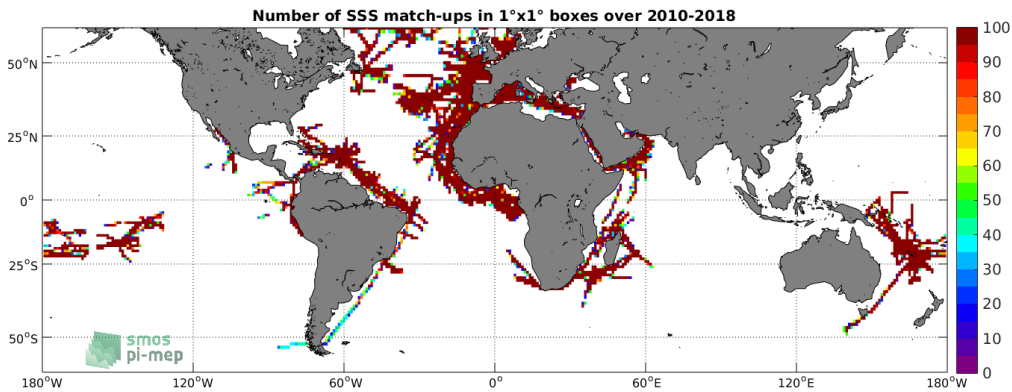
Figure 4: Number of SSS match-ups between TSG (GOSUD-Research-vessel) SSS and the SMOS SSS L3 v4 - 9 Days (CATDS-CECOS-LOCEAN) SSS product for the SMOS coastal zone (<800km) 60N-60S Pi-MEP region over 1^\circ \times 1^\circ boxes and for the full satellite product period.
