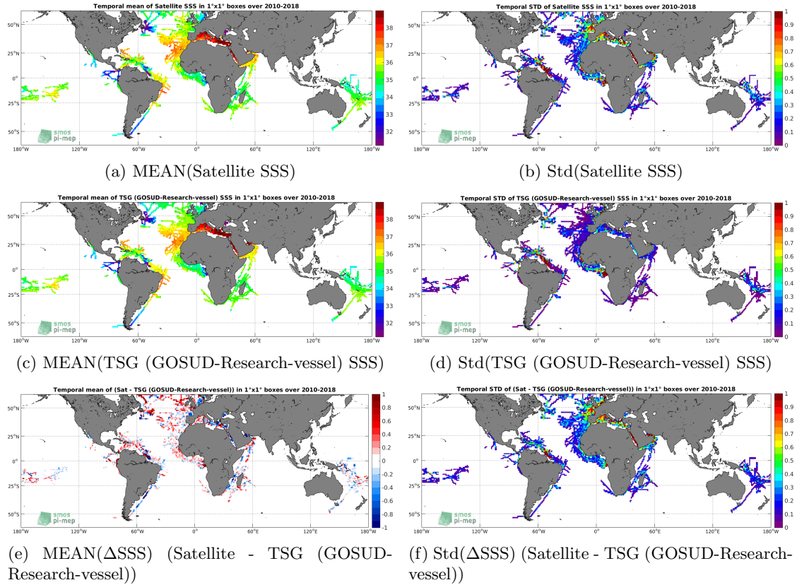
Figure 6: Temporal mean (left) and Std (right) of SSS from SMOS SSS L3 v4 - 9 Days (CATDS-CECOS-LOCEAN) (top), TSG (GOSUD-Research-vessel) (middle), and of \Delta SSS (Satellite - TSG (GOSUD-Research-vessel)). Only match-up pairs are used to generate these maps.
