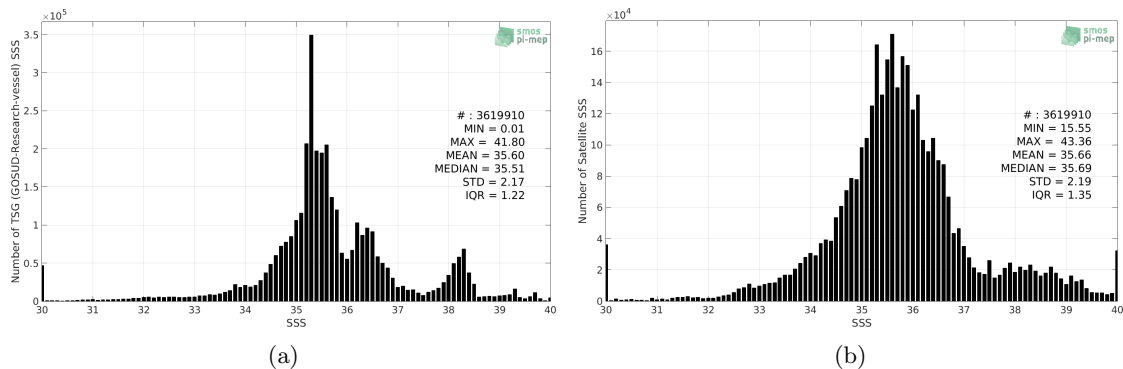
Figure 2: Histograms of SSS from TSG (GOSUD-Research-vessel) (a) and SMOS SSS L3 v4 - 9 Days (CATDS-CECOS-LOCEAN) (b) considering all match-up pairs per bins of 0.1 over the SMOS coastal zone (<800km) 60N-60S Pi-MEP region and for the full satellite product period.
