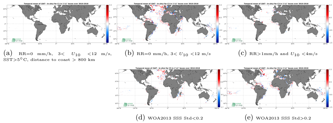
Figure 12: Temporal mean gridded over spatial boxes of size 1^\circ \times 1^\circ of \Delta SSS (SMOS SSS L3 v4 - 9 Days (CATDS-CECOS-LOCEAN) - TSG (GOSUD-Research-vessel)) for 5 different subdatasets corresponding to:RR=0 mm/h, 3 < U_{10} < 12 m/s, SST>5°C, distance to coast > 800 km (a), RR=0 mm/h, 3 < U_{10} < 12 m/s (b), RR>1mm/h and U_{10} < 4 m/s (c), WOA2013 SSS Std<0.2 (d), WOA2013 SSS Std>0.2 (e).
