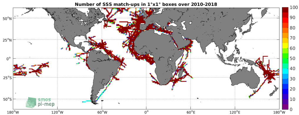
Figure 4: Number of SSS match-ups between TSG-GOSUD-Research-vessel SSS and the SMOS-L3-CATDS-CECOS-LOCEAN-V4-9DAYS-25KM SSS product for the SMOS coastal zone (<800km) 60N-60S Pi-MEP region over 1°x1° boxes and for the full satellite product period.
