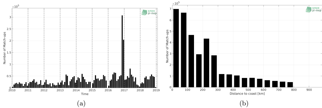
Figure 1: Number of match-ups between TSG-GOSUD-Research-vessel and SMOS-L3-CATDS-CECOS-LOCEAN-V4-9DAYS-25KM SSS as a function of time (a) and as function of the distance to coast (b) over the SMOS coastal zone (<800km) 60N-60S Pi-MEP region and for the full satellite product period.
