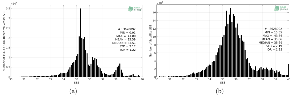
Figure 2: Histograms of SSS from TSG-GOSUD-Research-vessel (a) and SMOS-L3-CATDS-CECOS-LOCEAN-V4-9DAYS-25KM (b) considering all match-up pairs per bins of 0.1 over the SMOS coastal zone (<800km) 60N-60S Pi-MEP region and for the full satellite product period.
